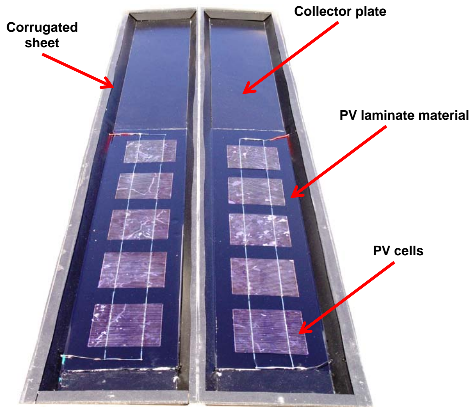
Figure 2: Unglazed BIPVT Colorcote prototype produced using adhesives
