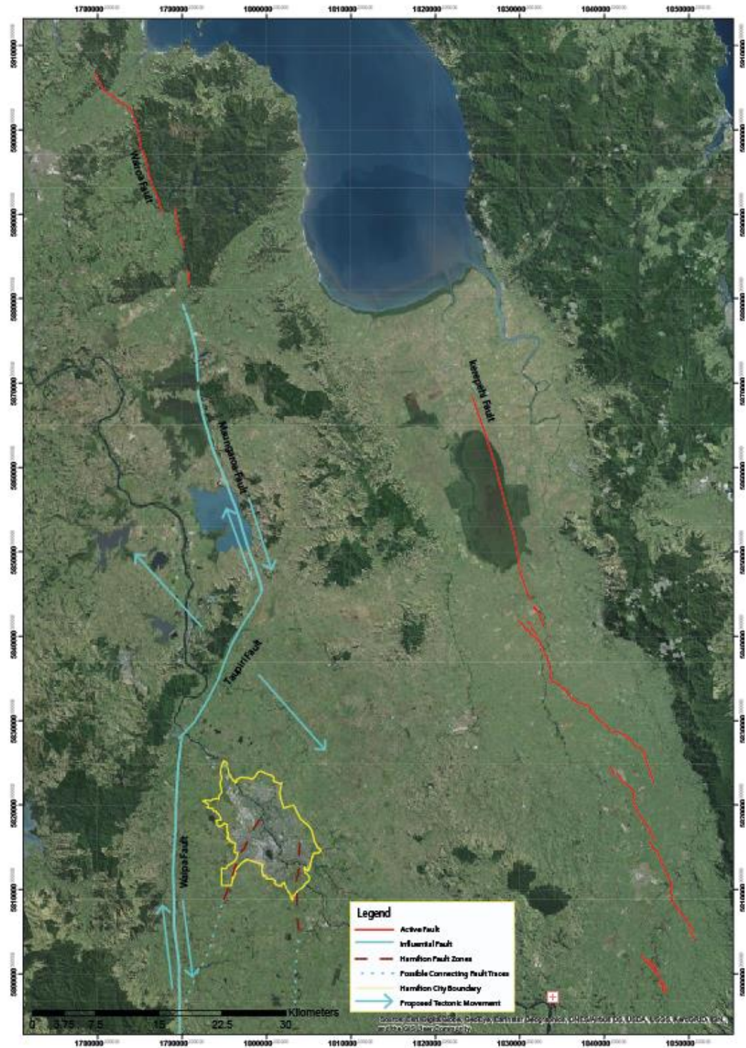
Figure 5.6. Map of proposed tectonic hypothesis for how and why the fault zones in Hamilton are forming. The influential faults, the Waipā and the Maungaroa Fault indicated by the light blue, are offset. The Taupiri Fault, also indicated by the light blue line, is the breached failure linking the two faults. Note that though the active Wairoa fault is not highlight blue, it has a similar orientation to the Maungaroa Fault, indicating that it too could be contributing to the formation of fault zones in Hamilton.
