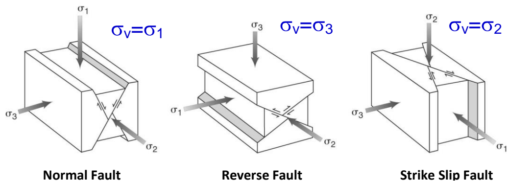
Figure 2.4. Diagram of Fault systems and their associated stress regime orientation. Fault represents a response of rock to shear stress, type is determined by which primary stress is oriented vertically.
