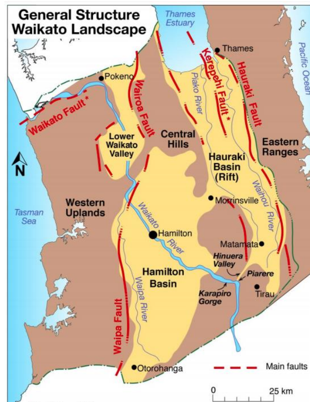
Figure 1.1. Map of the Hamilton Basin from Lowe (2010) showing the basins location within the central North Island. Fault lines within the region are indicated by the red lines and the Waikato River is indicated by the blue.
