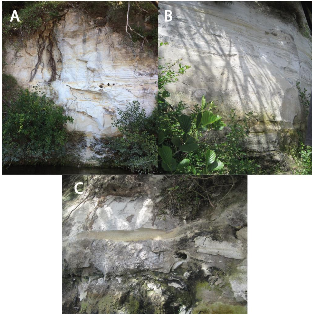
Figure 4.24. Photographs of outcrops found near and at Location 18. A) southernmost outcrop with erosion pipes in silt layer. B) Outcrop of R2S4 located on the southern section of Location 18. C) Outcrop near Day's Park between Location 18 and Station M. Stratigraphic log taken from this outcrop.
