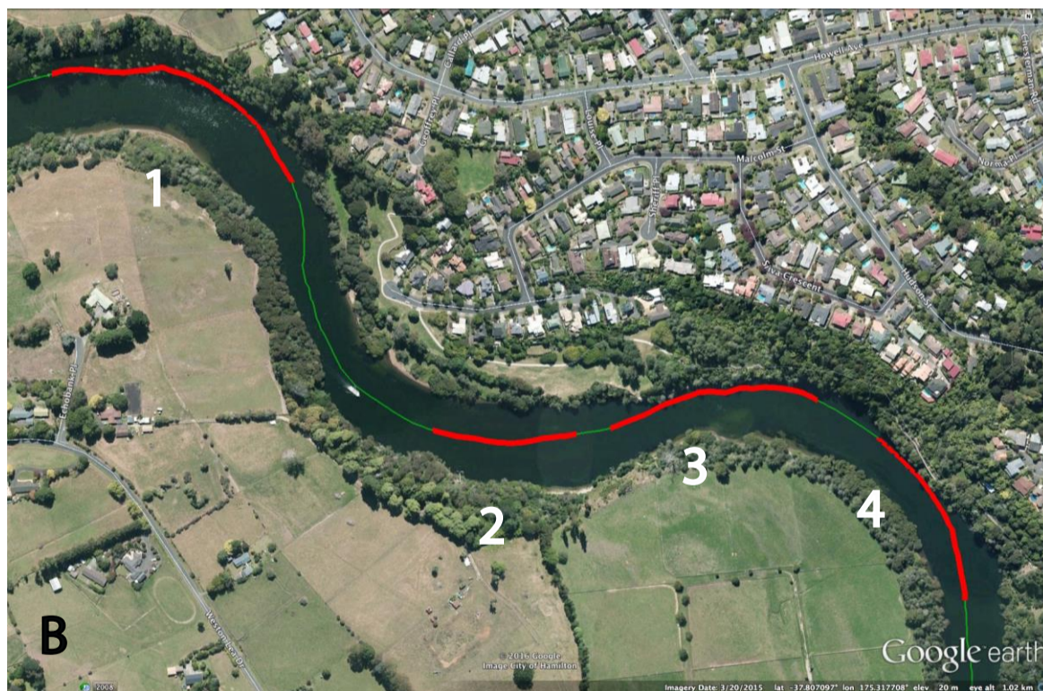
Figure 4.20. Seismic Survey data taken along Bends 3 and 4 at Hammond Park. Location of each specific survey image is marked by number 1-4 in the map below. Image 3 was taken along the transect of the scourhole seen in the 3D multibeam image in 4.19-2 and shows knickpoint with discontinuity. No transect was taken along the region between Location 12 and 13, but images 1 and 2, taken up and down river of that region, show a discontinuity. Image 2 shows a change in the density of the riverbed geology from less dense in south and more dense in the north.
