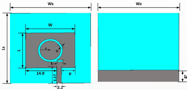
Fig. 1. Geometry of the proposed antenna: (left) top view, and (right) bottom view. All dimensions are in mm.
