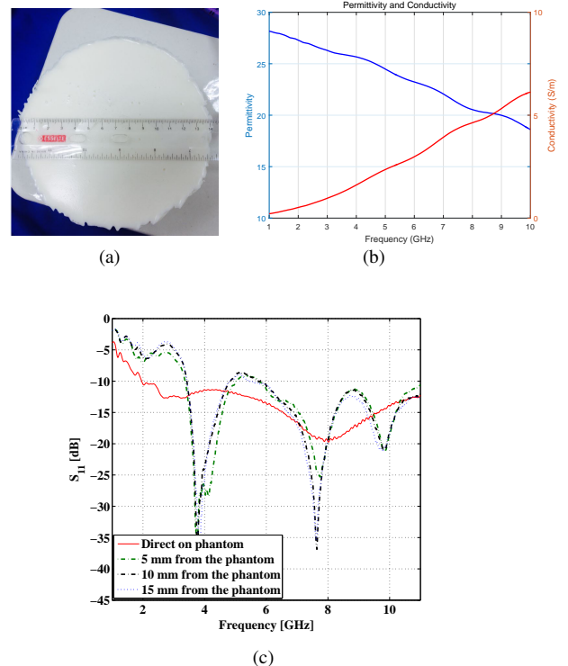
Fig. 9. Summary of our breast phantom measurements. (a) Photo of the homogeneous breast phantom; (b) Plot of its tissue-mimicking dielectric properties vs frequency; (c) Measured S_{11} when the antenna is placed in close (varying) distances to the phantom.
