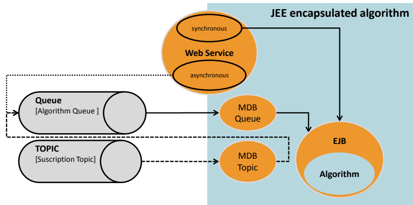
Figure 2: Structure of an encapsulated algorithm.
