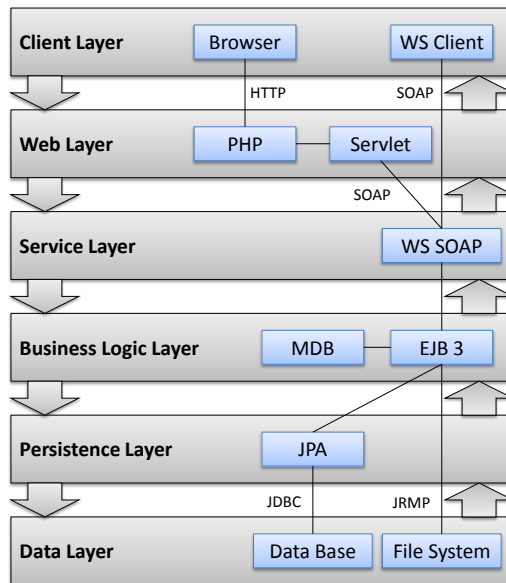
Figure 1: DOCODE system's layers diagram.
