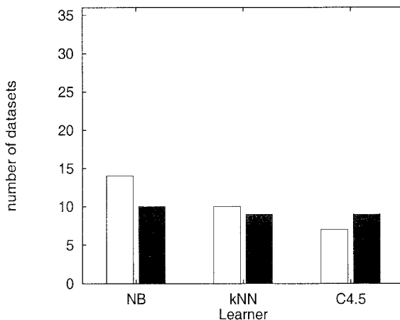
Figure 1: Results of paired t -tests ( p = 0.05 ): left bar for each learner indicates how many times feature selection significantly improves performance; the right bar indicates how many times using the full feature set significantly outperforms feature selection.
