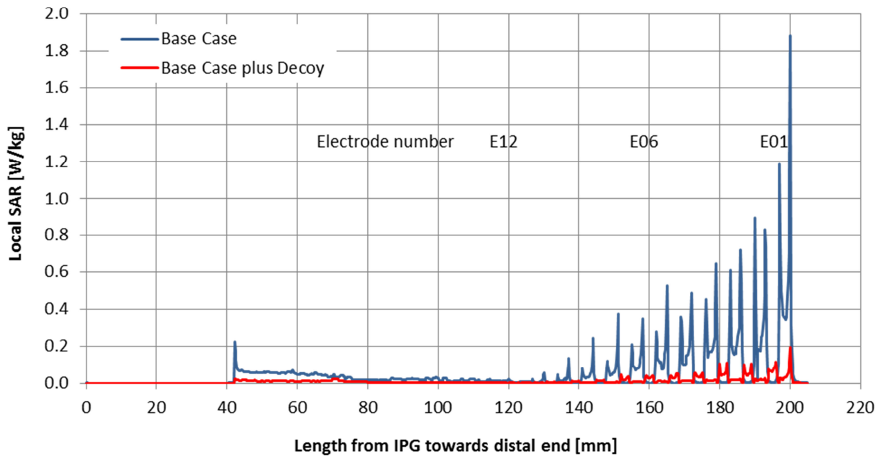
Figure 2 - Local SAR in saline solution normalised to 1 V/m of the exciting electrical field for a spinal cord stimulator with 12 electrodes at the distal end and for a worst case lead length of 200 mm
