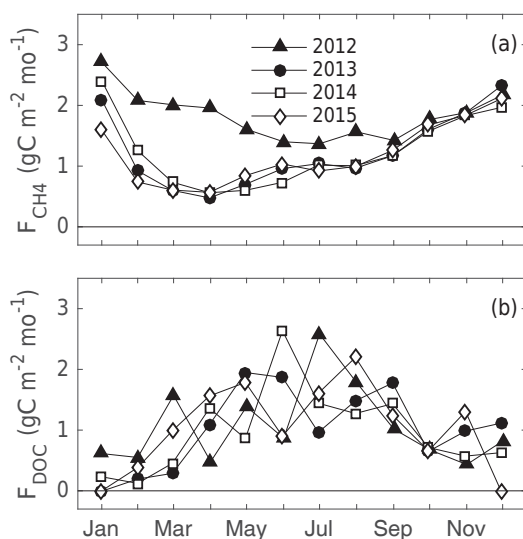
Figure 3. Monthly total non-CO 2 -C flux components at Kopuatai bog over the 4 measurement years. (a) Methane flux ( F_{\text{CH}_4} ), (b) dissolved organic carbon export ( F_{\text{DOC}} ).
