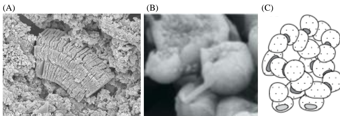
Figure 2. Scanning electron micrographs of (A) book and (B) mushroom-cap morphologies of halloysite. (C) Inferred framework network of mushroom cap clay minerals. Image credits: (A) Helen Turner, (B) and (C) from Kluger et al. (2017).
