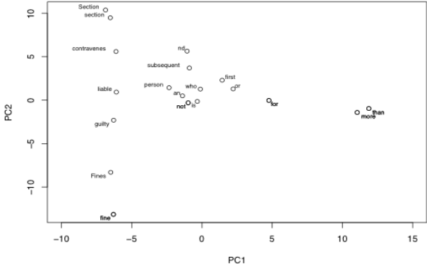
Figure 1: Words vectors from the previous example visualized by plotting their first two principle components.
