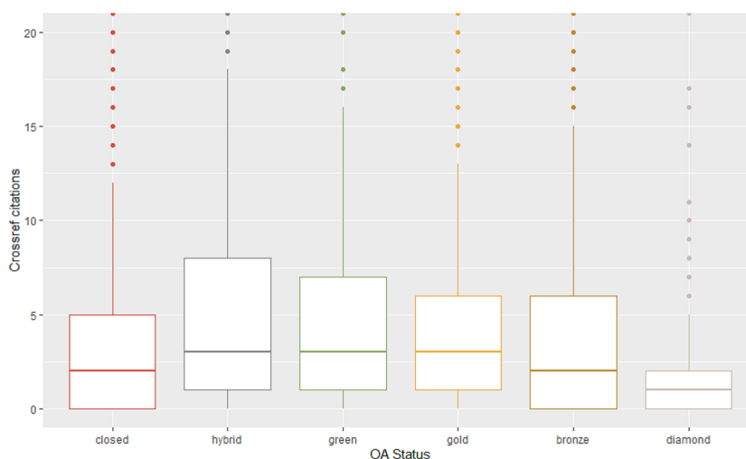
Figure 2 Crossref citations for different types of access. This boxplot compares the distribution of citations for each type of access. Citations, drawn from Crossref, are indicated on the Y axis. Average citation rates for each type are indicated by the horizontal line in each box. Each category had a number of outliers (depicted as dots). The graph is cropped at 20 citations on the Y axis to focus on the groupings of citations in the 0–10 range.
