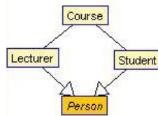
Fig. 1. Class Diagram derived in USE
