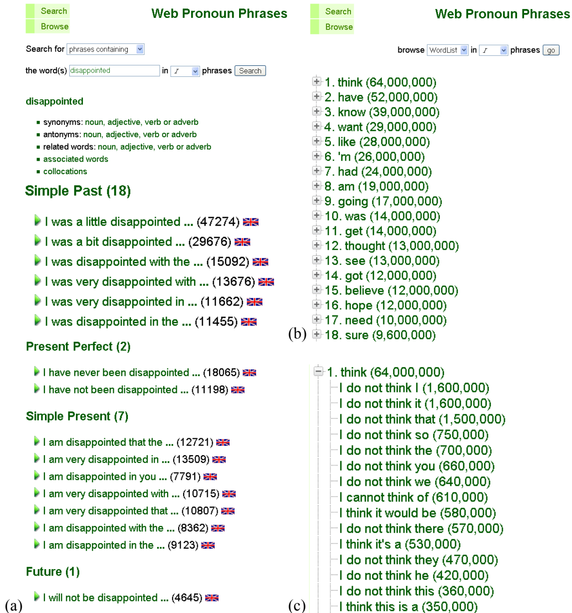
Figure 3. Searching and browsing the pronoun phrase collection
