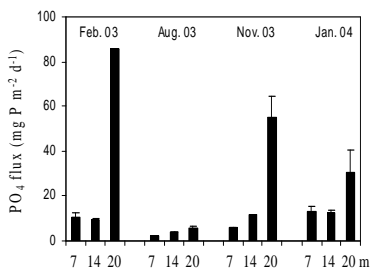
Fig 5. Mean phosphate fluxes from 4-day in situ benthic chamber incubations for four periods in 2003-4 at three stations of depths denoted on the horizontal axis.
