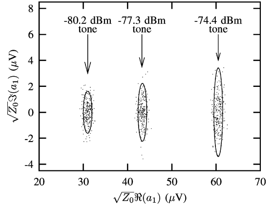
Fig. 5. Plot of the samples used to calculate the variance of the measured -80.2 -, -77.3 -, and -74.4 -dBm tones. The measurements used for this plot are from a lower amplitude multitone signal than that plotted in Fig. 3. A 95% confidence region for the mean of each tone is superimposed on the sample points (see [14]). The covariance matrix element V_{11} is proportional to the width and V_{22} is proportional to the height of the oval defining the confidence region. For low power levels, the width ( V_{11} ) remains fairly constant, while the height ( V_{22} ) increases with increasing signal amplitude.
