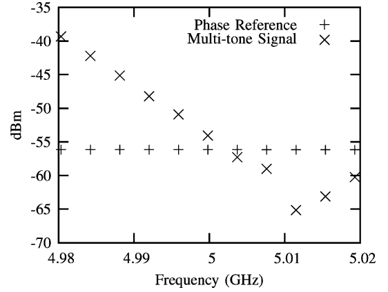
Fig. 3. Measured magnitude spectrum of a multitone signal and magnitude spectrum of the phase reference. The phase reference clock frequency was set to 3.9 MHz.
