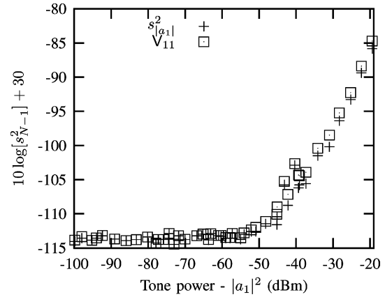
Fig. 6. Plot of the sample variance of the magnitude s^2_{|a_1|} and the sample variance of the real part V_{11} when the phase reference is driven by the Agilent E4437 signal generator. The variance of the magnitude is constant at low tone powers and then increases with increasing tone power above -55 dBm. This suggests that the magnitude |a_1| does not have a Rice distribution. The sample variance of the real part V_{11} is highly correlated with the sample variance of the magnitude s^2_{|a_1|} .
