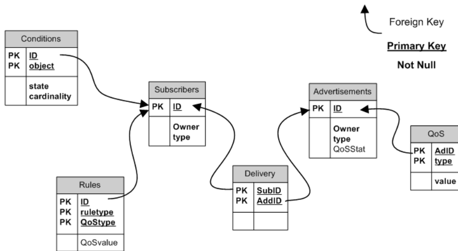
Figure 9: Database Layout
