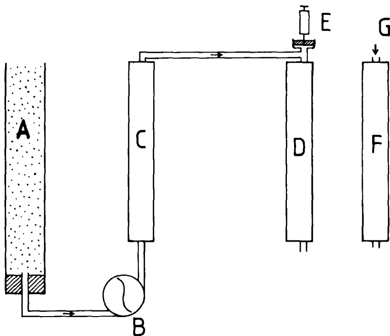
Fig. 1 Diagrammatic representation of gas flow system. A: carbasorb column; B: air pump; C: gas flow meter; D: analysis cell of IRGA; E: gas sample injection point through suba seal; F: reference cell of IRGA; G: CO 2 -free air from internal supply in IRGA. Gas flow rates were 900 ml min -1 through analysis cell, 180 ml min -1 through reference cell.
