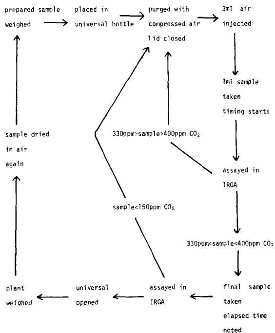
Fig. 3 Standard assay routine indicating decision points necessary to maintain a constant CO 2 concentration range. The decision points do not need to be applied during respiration assays.
