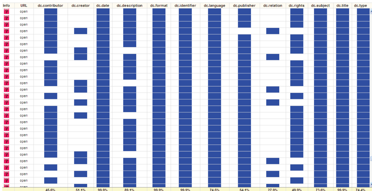
Figure 3. Part of a visualisation of 6000 OAI Dublin Core records from MINDS @ Wisconsin (two empty elements are hidden)
