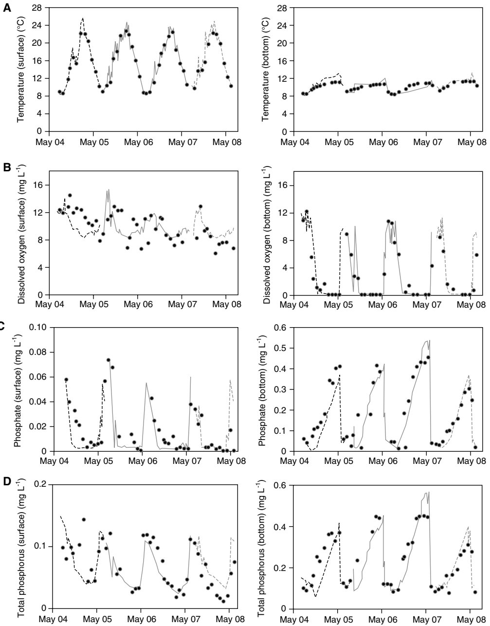
Figure 3 Comparison of model simulation results (grey lines) against field observations (black circles) in the surface (0 m) and bottom (14 m) waters of Lake Okaro during the calibration period (solid grey line) and validation periods (dashed grey and black line). A , Temperature. B , Dissolved oxygen. C , Phosphate. D , Total phosphorus.
