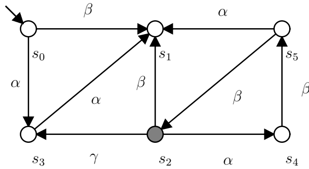
Figure 2.8: An automaton with blocking states.
