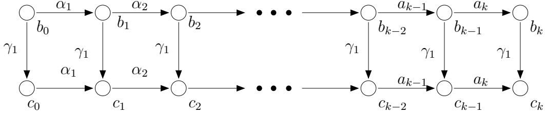
Figure 3.6: Example of independent events remaining enabled.
