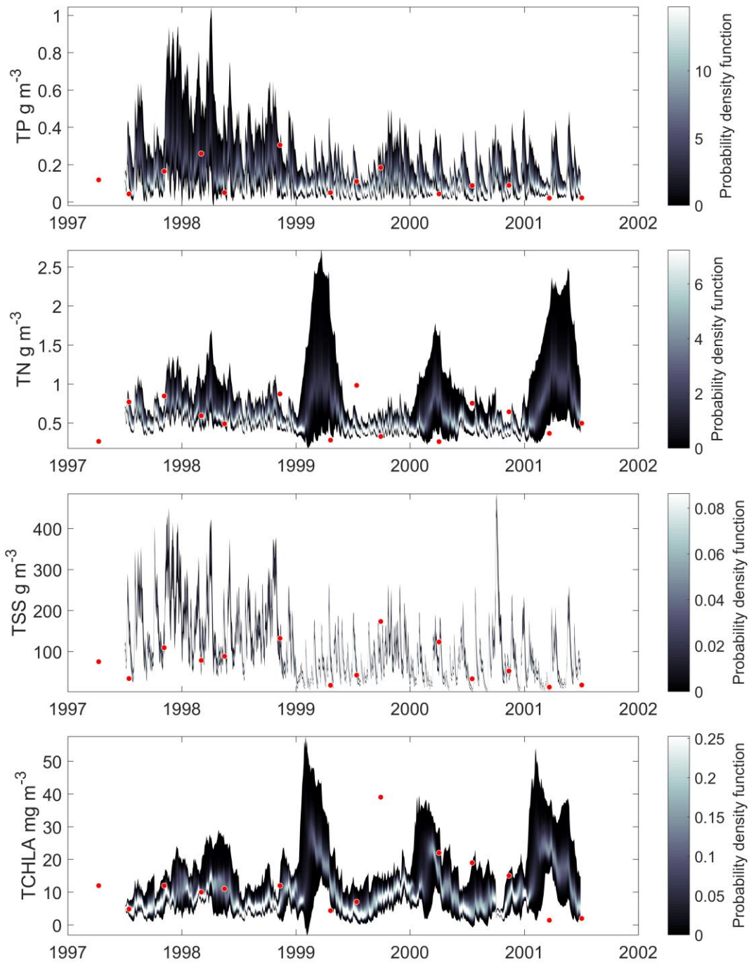
Figure 44. Probability density plots show the range of water quality related outputs generated from plus or minus 5% if sensitive parameters. Measured in situ data is plotted with a red closed circle. TCHLA is total chlorophyll a, TSS is total suspended sediment, TP is total phosphorous and TN is total nitrogen.
