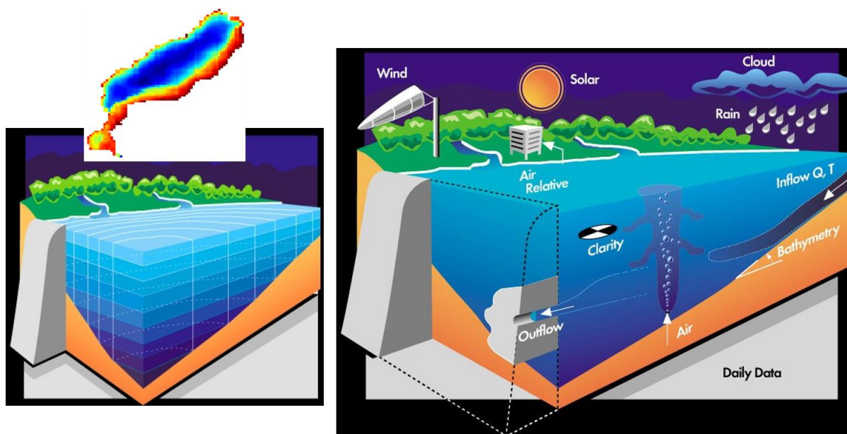
Figure 8. Schematic of the 3-D model grid structure whereby the model accounts for both horizontal and vertical variation in simulated variables such as water temperature and water quality.
