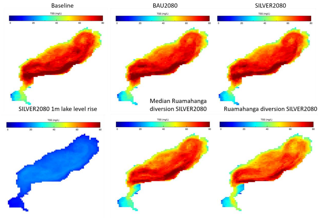
Figure 42. Simulated total suspended solids concentrations in Lake Wairarapa using three-dimensional models (AEM3D). BAU is business as usual.
