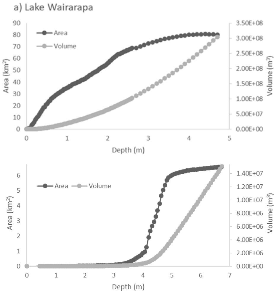
Figure 13. Hypsographic curves of area and volume vs. depth for; a) Lake Wairarapa and b) Lake Onoke.
