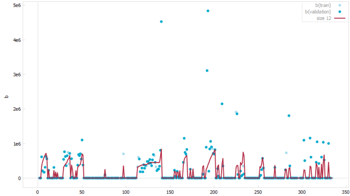
Appendix Figure 1. Barrage inflow estimations (redline) compared to in situ measurements (blue dots). Correlation Coefficient = 0.58, mean absolute error=122125.75 m 3 /day.
