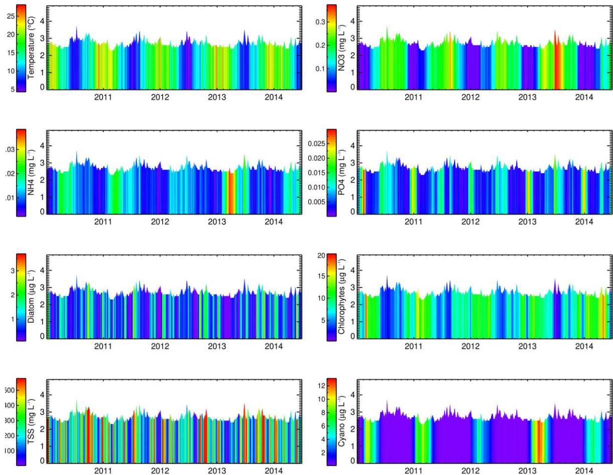
Figure 22. Contour plot of 1-D simulated water quality variables for Lake Wairarapa. The left axis is elevation from the lake bottom (m). Nitrate is (NO 3 -N), Ammonia (NH 4 -N), Phosphate (PO 4 -P) and total suspended solids (TSS).
