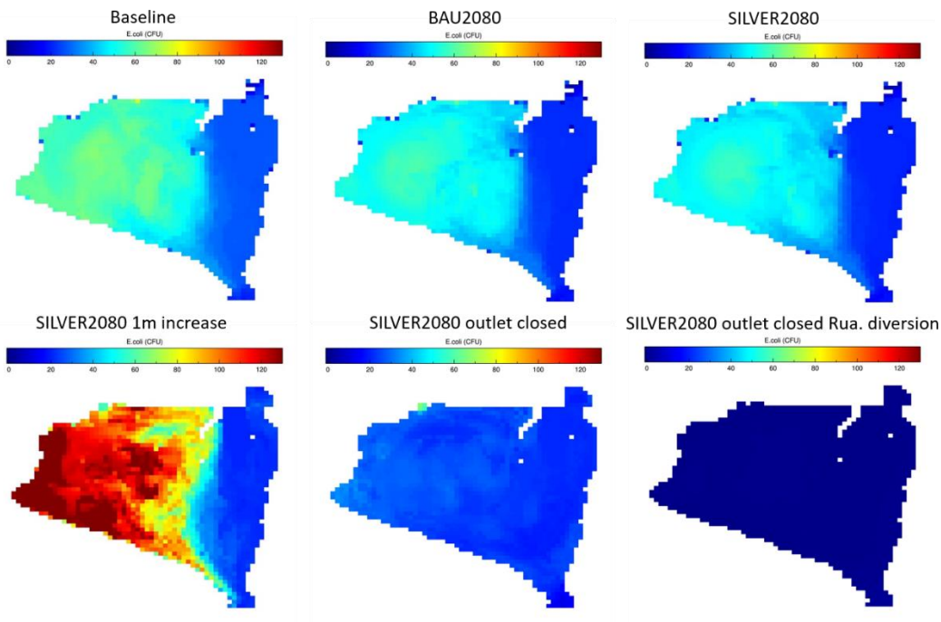
Figure 35. Median 3-D simulated E. coli concentration in Lake Onoke over a 91 day period beginning 1 Jan 2012 at 12pm. The scale runs from 0 to 130 CFU, with median 130 CFU being the swimmability boundary between excellent and intermittent.
