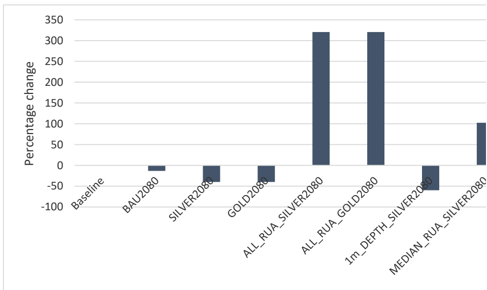
Figure 32. The 1-D simulated percentage change in E.coli concentrations (y axis) in Lake Wairarapa comparing Baseline to 2080 scenarios (x axis).
