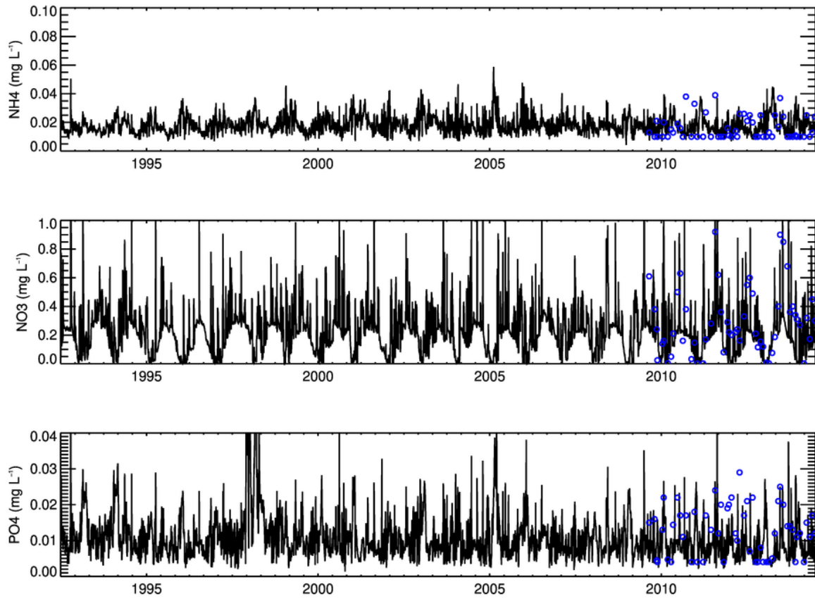
Figure 28. Surface water quality for Lake Onoke. Black line is the simulated values, and blue open circles are observed values. Note that field data are only available from 2009 in lake Onoke.
