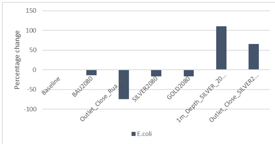
Figure 33. The 1-D simulated percentage change in E. coli concentrations in Lake Onoke comparing Baseline to 2080 scenarios.
