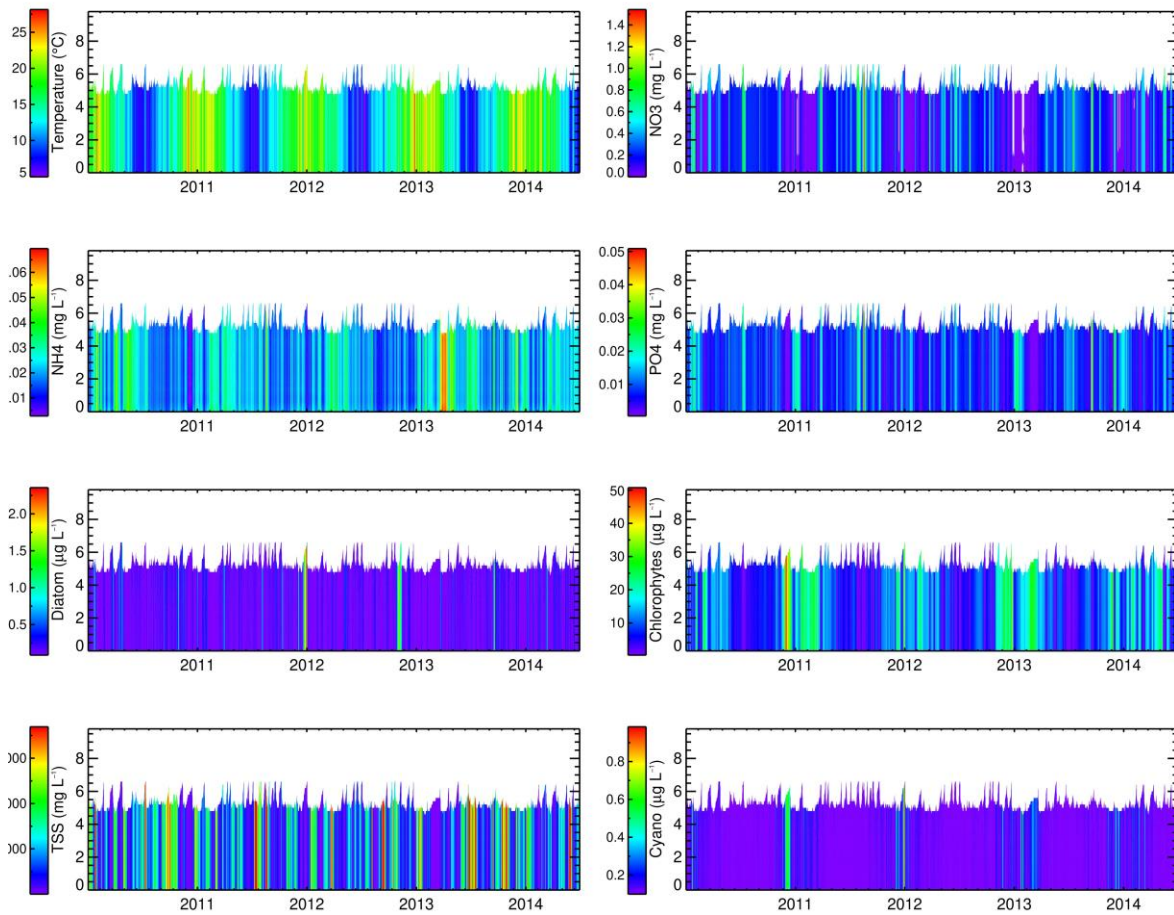
Figure 30. Contour plot 1-D simulated water quality variables for Lake Onoke The left axis elevation from the lake bottom (m). Nitrate is (NO 3 -N), Ammonia (NH 4 -N), Phosphate (PO 4 -P) and total suspended solids (TSS).
