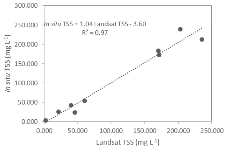
Figure 15. Comparison of in situ TSS to Landsat estimated TSS ( \text{mg L}^{-1} ) using a semi-analytical relationship (Fig. 14).
