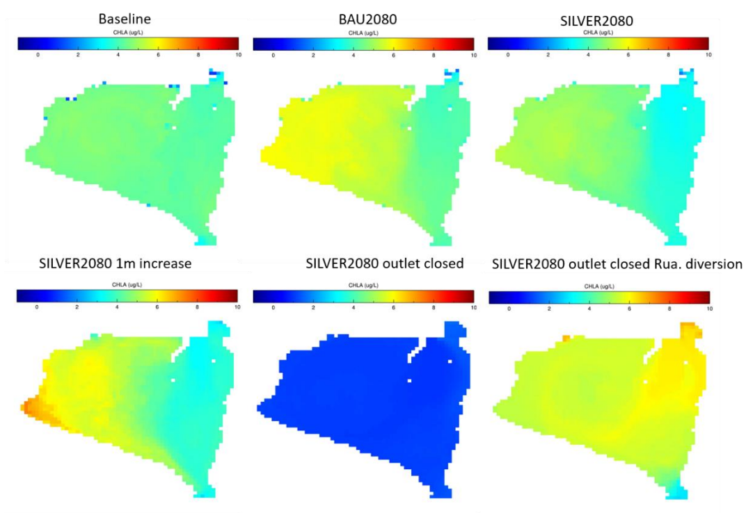
Figure 41. Simulated total chlorophyll a concentrations in Lake Onoke using three-dimensional modeling (AEM3D). BAU is business as usual.
