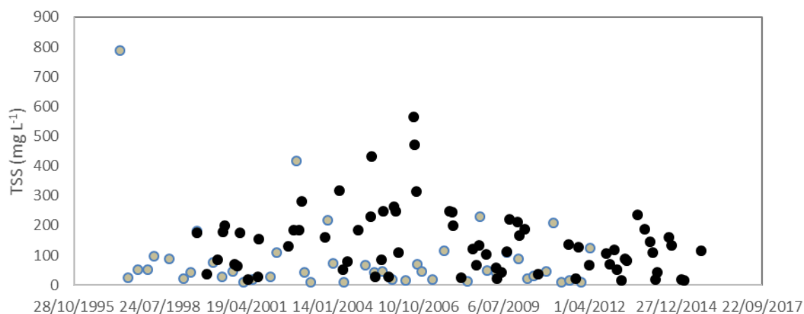
Figure 16. Time series of total suspended solids (TSS) at Lake Wairarapa Site 1 using Landsat (black filled circles), compared to those measured in situ (grey filled circles). Landsat TSS explained 97% of the variation of in situ TSS (see Fig 14).
