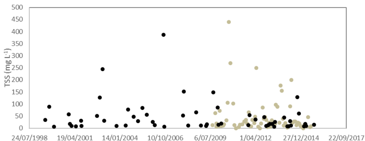
Figure 17. Time series estimation of total suspended solids (TSS) at Lake Onoke using Landsat (black filled circles), compared to those measured in situ (grey filled circles). Landsat TSS explained 97% of the variation of in situ TSS (see Fig 14).
