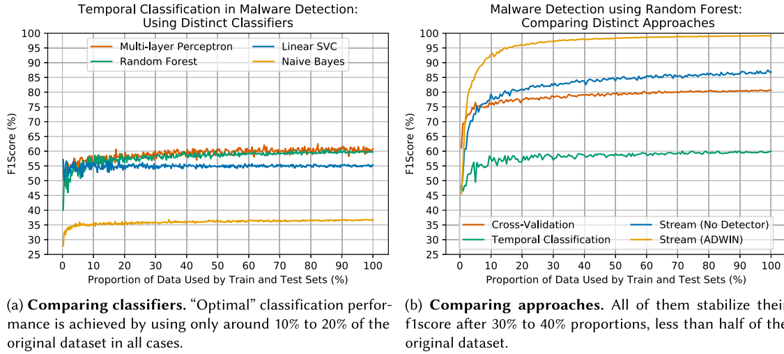
Fig. 6. Dataset size definition in terms of f1score. In both experiments a similar behavior is seen, with a certain stability in classification performance after using only a given proportion of the original dataset.
