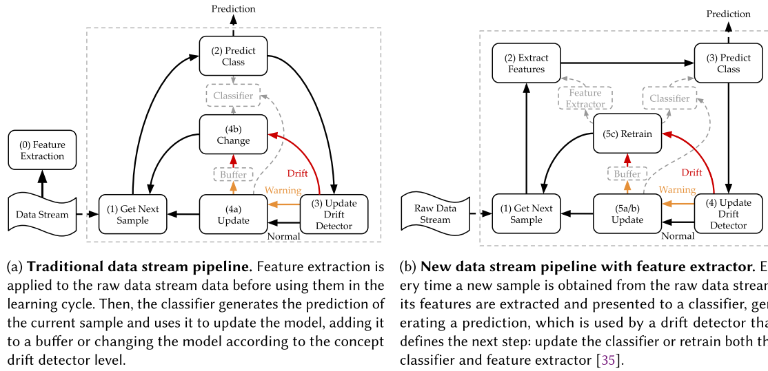
Fig. 8. Data stream pipeline. Comparing the traditional data stream pipeline with possible mitigation that adds the feature extractor in the process, generating updated features as time goes by [35].
