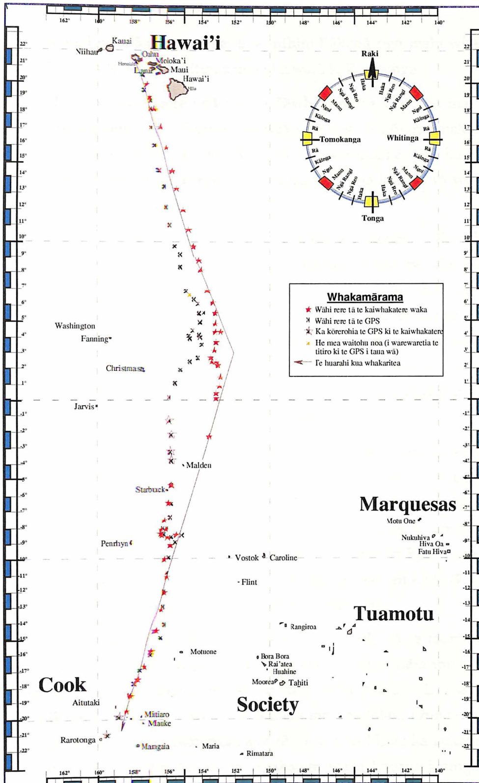
Whakaahua 33: Te Ara Moana i Takahia e Te Aurere
