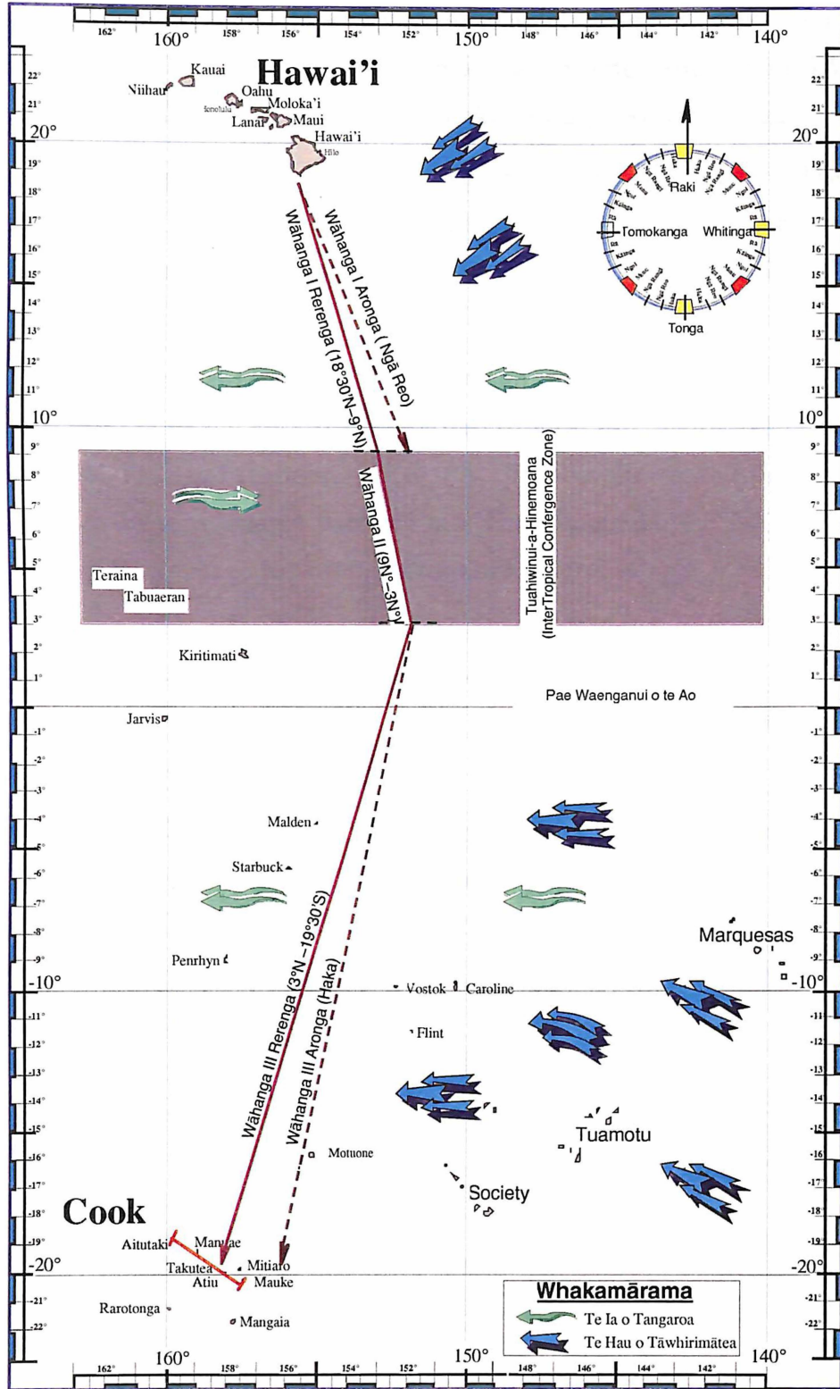
Whakaahua 23: Te Ara Moana I Whakaritea
