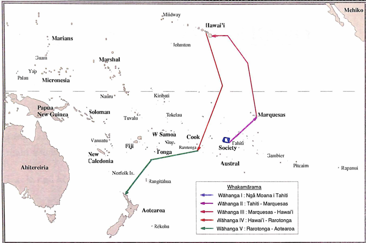
Whakaahua 6: Ngā Rerenga a Te Aurere i te tau 1995
