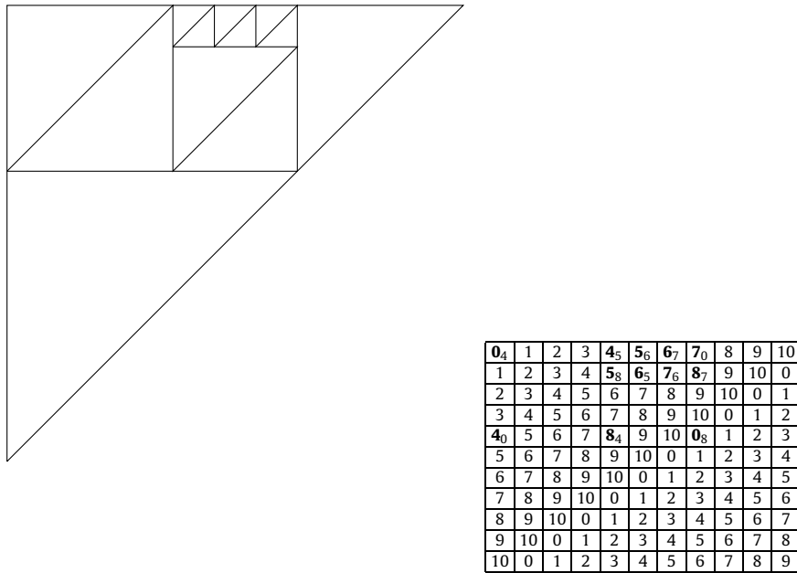
Fig. 2. A good tessellation of \mathcal{E}_{11} (reflected on the x -axis) and the corresponding Latin trade in B_{11} .
