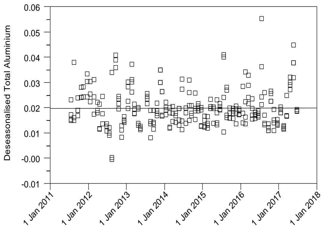
Figure 2. Top. Seasonal trend in water column total aluminium concentrations in Lake Rotoroa from July 2011 – June 2017 and, Bottom. Deseasonalised total aluminium concentrations for the same period.
