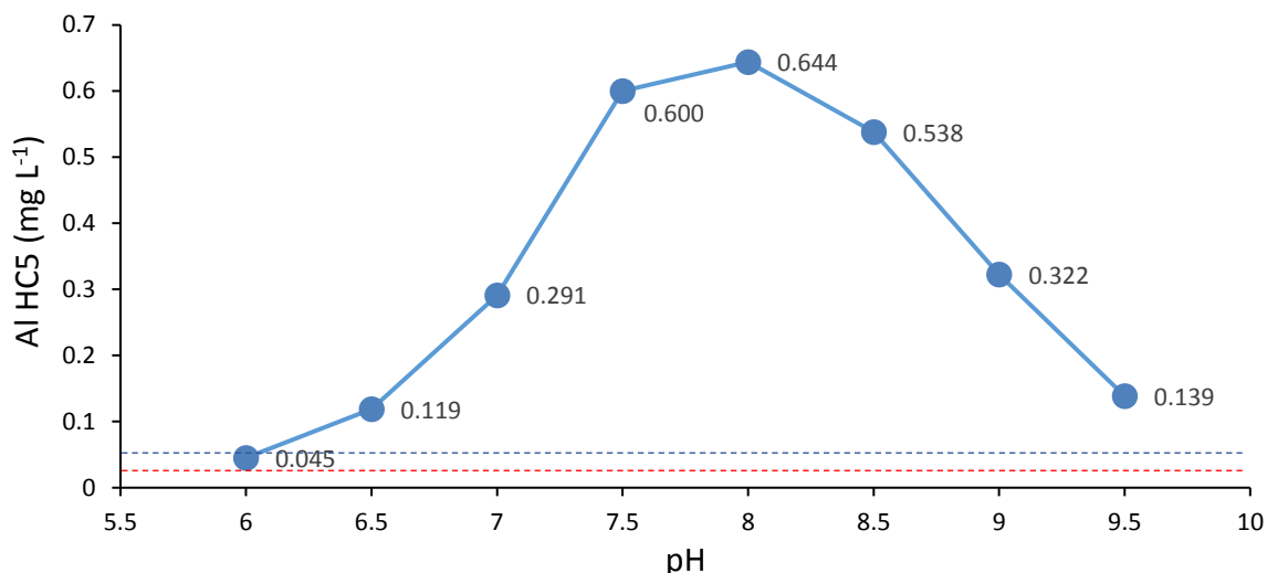
Figure 4. Total aluminium 5% hazardous concentrations (HC5) for Lake Rotorua under differing pH values based on mean dissolved organic matter concentration of 2 mg L -1 and mean water hardness of 14 mg L -1 (as CaCO 3 ). HC5 values were calculated using DeForest et al. (2018) multiple linear regression models. The blue dashed line indicates ANZECC 2000 trigger value for dissolved aluminium in freshwater systems, and the red dashed line indicates mean total aluminium concentration for Lake Rotorua.
