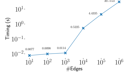
Figure 4: ARES-Static timings on CIC-IDS2017 dataset as the number of edges increases
