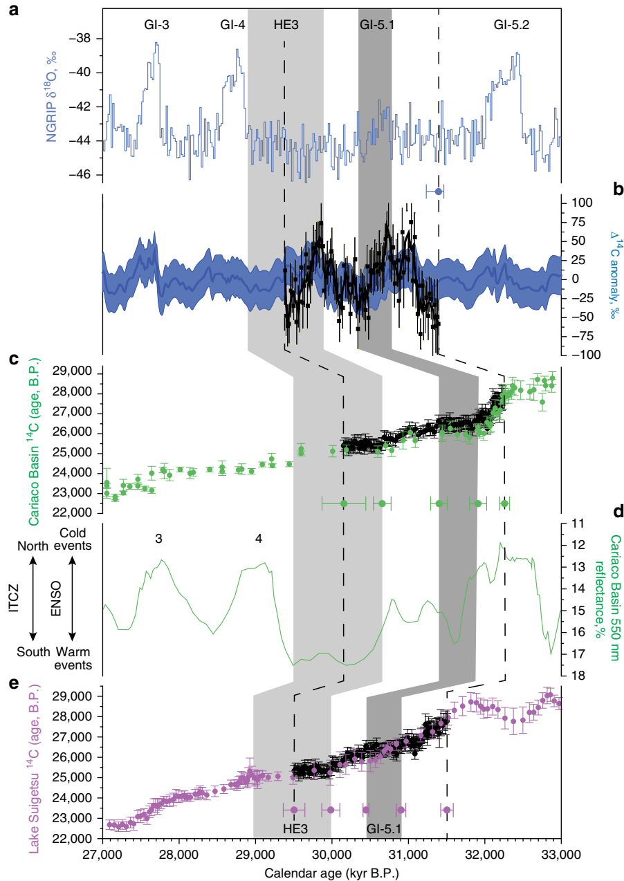
Fig. 1 High-precision alignment of 2000-year long Finlayson 8 kauri tree 14 C measurements to key datasets. Bidecadal \Delta^{14}\text{C} data through the kauri tree (black filled circles with 3 point-running mean) compared to the Greenland (blue) \delta^{18}\text{O} and detrended 10 Be flux-derived \Delta^{14}\text{C} anomalies 10, 16 a, b . Comparison of kauri 14 C age measurements and Cariaco Basin 14 ( c and d ; green symbols) and Lake Suigetsu 13 ( e ; purple symbols) radiocarbon ( 14 C) calibration data sets on the modelled Hulu Cave and SG06 2012 timescales, respectively. Green reflectance changes preserved in the tropical Atlantic Cariaco Basin marine sequence provide a measure of the meridional migration of the Intertropical Convergence Zone (ITCZ; d ). Greenland Interstadials are numbered; Heinrich Event 3 (HE3, based on the climatostratigraphic position in MD95-2040) 17 and Greenland Interstadial 5.1 (GI-5.1) are shown by light and dark grey columns, respectively. The dashed lines denote the time range captured by the 2000-year kauri 14 C record used in this study 10 . Calendar age uncertainties for synchronization of records shown at 2\sigma (95% confidence limits)
