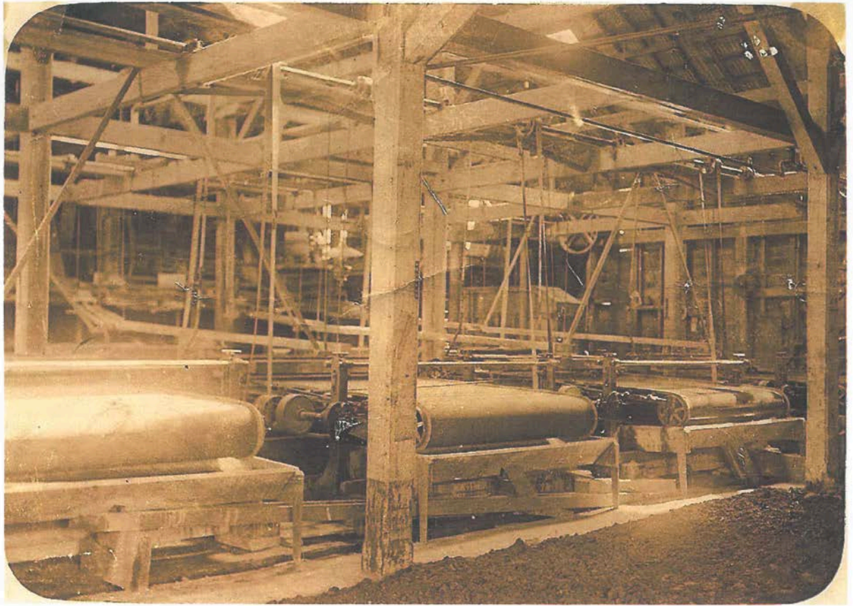
Figure 6: E.H. Hardy, the inside of his Waiorongomai battery, n.d., c. 1900, David Calder Hardy Collection; used with permission.
