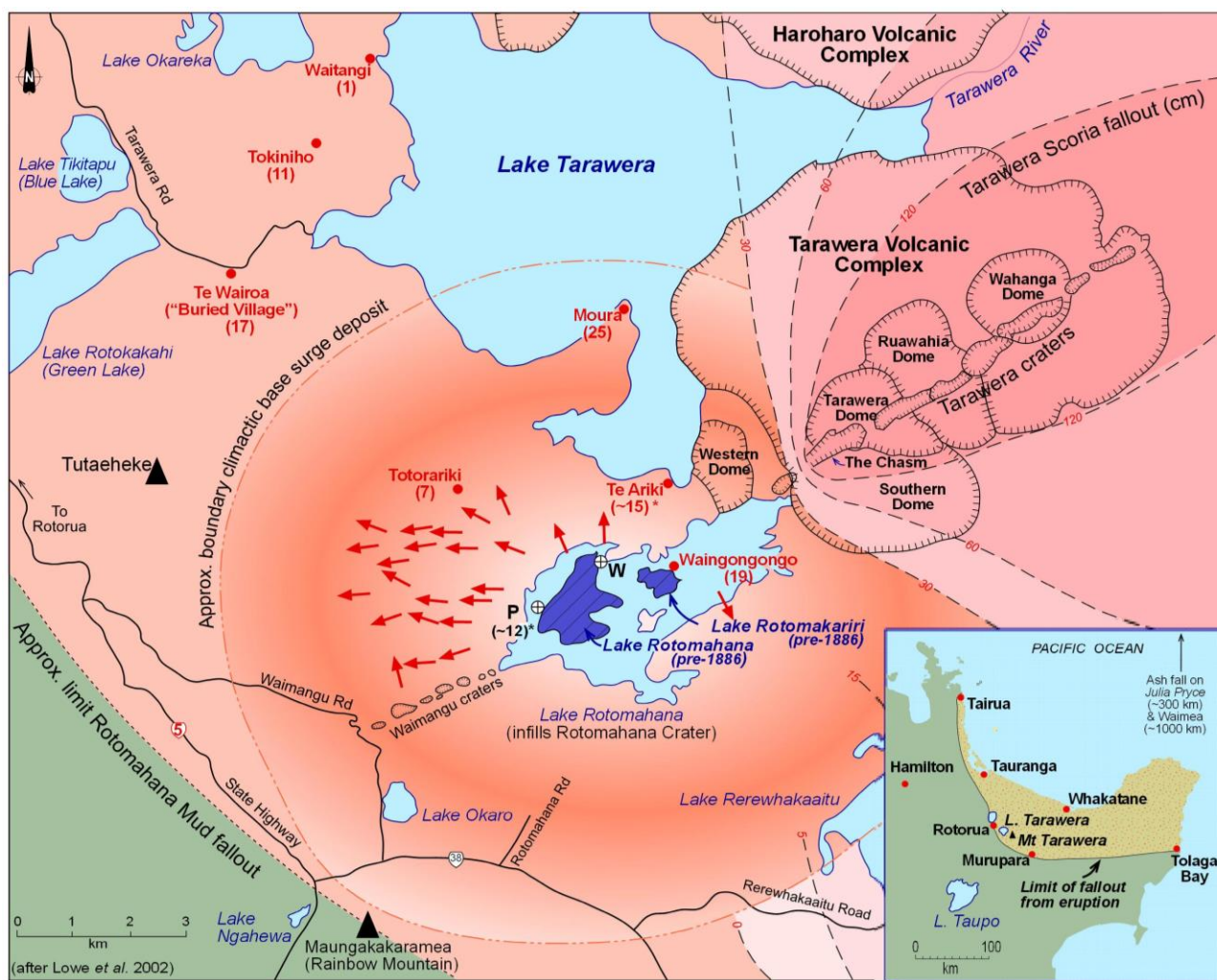
Figure S6 Map of Tarawera area showing locations of the main craters of the 10 June 1886 fissure eruption across Tarawera Volcanic Complex, Rotomahana Crater (including pre-eruption lakes Rotomahana and Rotomakariri), and Waimangu craters (after Lowe et al., 2002). Locations of villages and associated fatalities (numbers in parentheses, total ~120) are based on Keam (1988) and Lowe et al. (2001) (there was an additional death at an unknown locality). Fatalities were all Māori apart from six Europeans at Te Wairoa and one European and three Māori at Waingongongo. On the night of the eruption nearly half of Te Ariki's 27 residents were camped at Pink Terrace (Te Otukapuarangi). Inset shows eastern North Island and documented limits of tephra fallout from the eruption (based on maps by Thomas, 1888). Ash fell on several ships at sea, the farthest being Julia Pryce (c. 300 km) and S.S. Waimea (c. 1000 km) north of North Island (Keam, 1988). Lorrey and Wolley (2018) used historic data recorded during Ferdinand Hochstetter's 1859 survey to locate the sites of Lake Rotomahana's former sinter terraces (see also de Ronde et al. 2016, 2019; Keam, 2016; Keir, 2019).
