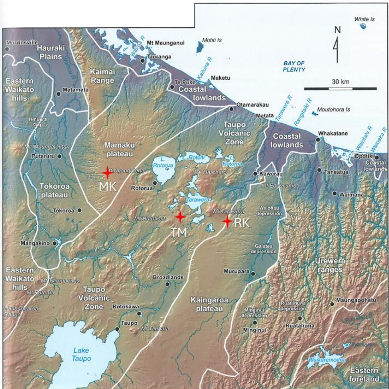
Figure S2 Topographic relief model illustrating the broad physiographic regions in the Bay of Plenty-Rotorua-Taupō region. The ‘geomorphic’ Taupō Volcanic Zone (TVZ) comprises an area of largely volcanic hills and lakes and covers a similar area (but not exactly equivalent) to the ‘volcanologic’ TVZ (defined by vent locations only) (from Leonard et al., 2010). The locations of the training and competition section/pits for the soil judging competition are shown as red stars: MK, Mamaku Plateau; RK, Rerewhakaaitu (on eastern margin of TVZ/western margin of Kaingaroa Plateau); TM, Tumunui area (Highlands Rd) (competition profiles).
