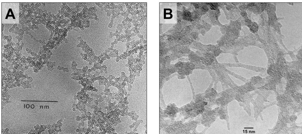
Figure S11 Micrographs of (A) allophane and (B) imogolite (external nanotube diameter is \sim 2 nm) (from McDaniel et al., 2012, after Parfitt, 1990, 2009).
