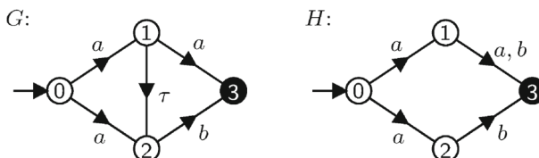
Fig. 7 Two weakly observation equivalent FSMs (Malik and Leduc 2013)
