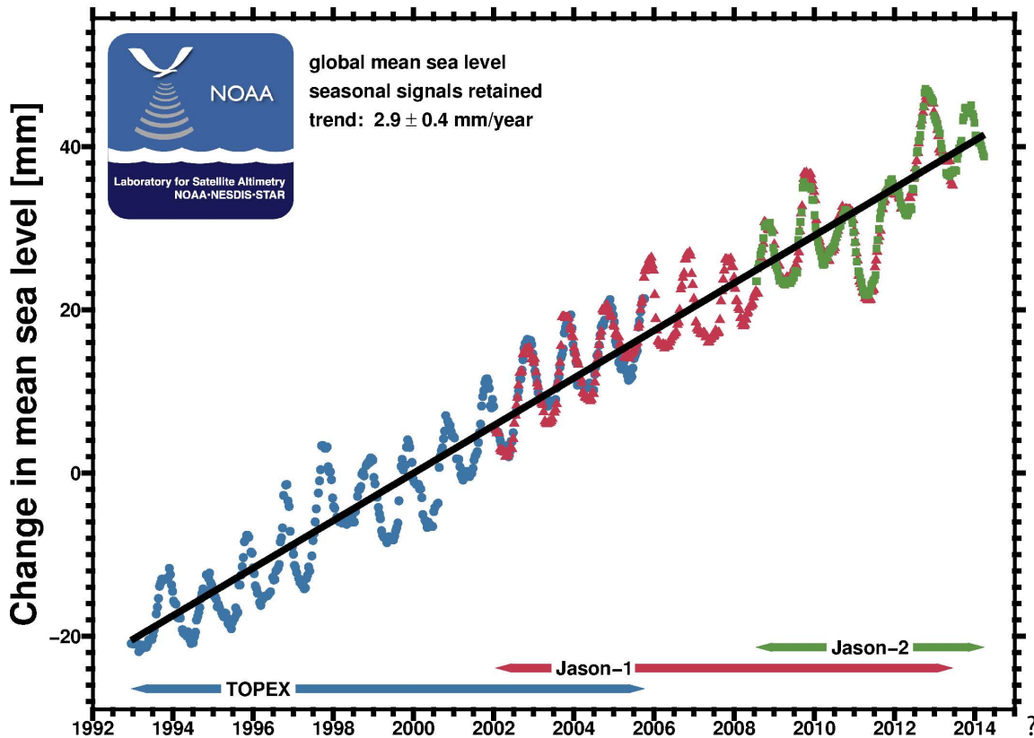
Figure 5: NOAA satellite altimetry, global sea-level change since 1992. Dataset composite, collected from successive satellites (coded in colour), and plotted monthly without seasonal corrections. http://www.star.nesdis.noaa.gov/sod/lisa/SeaLevelRise/LSA_SLR_timeseries.php .
