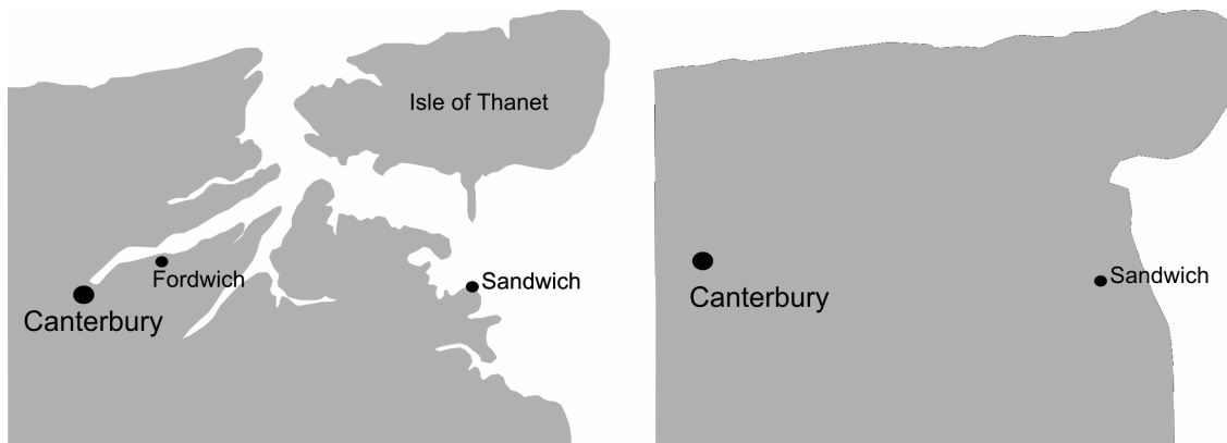
Figure 2: Geography of eastern Kent. Left: As it was between the first and fifteenth centuries. Right: As it is today.
