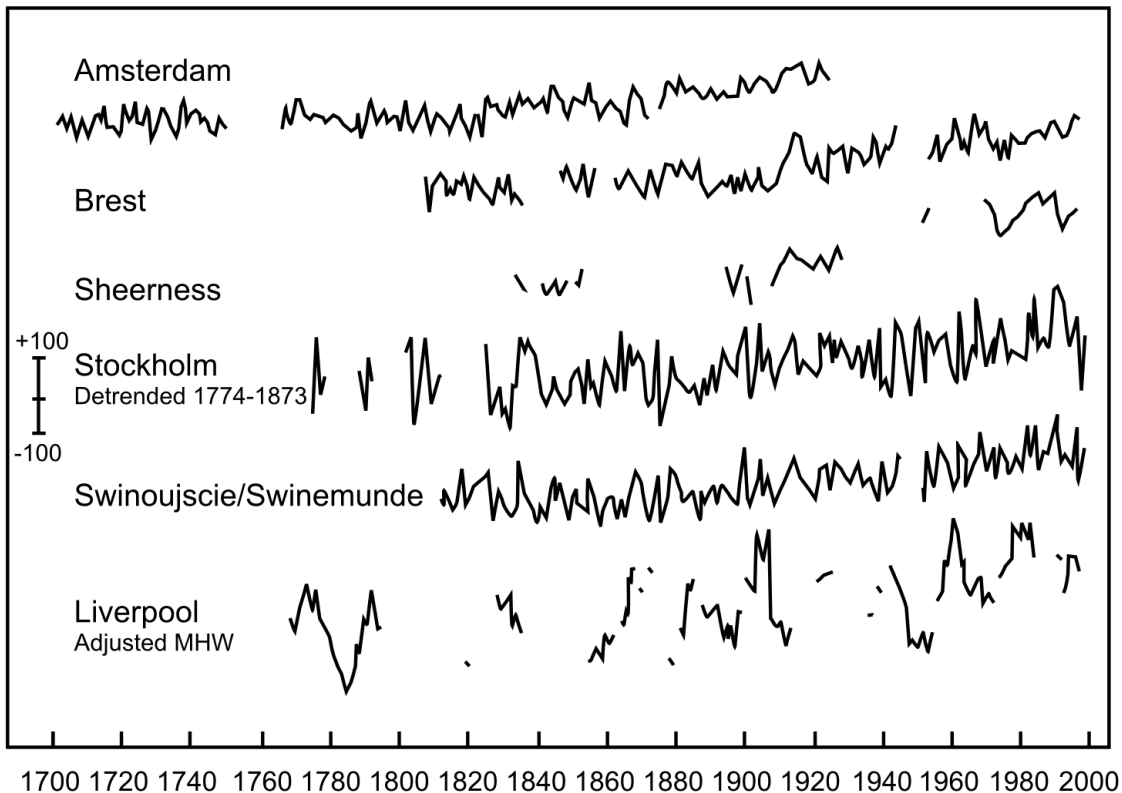
Figure 4: Long, northern hemisphere tide-gauge records of sea-level change, 1700–2000. After Hadley Centre and IPCC, TAR.
