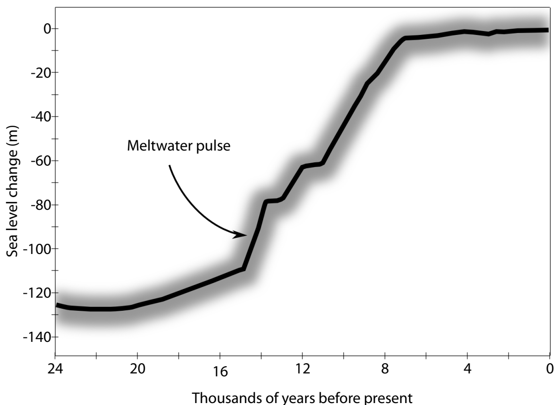
Figure 3: Reconstructed global sea-level since the last glacial maximum, 20,000 years ago, based on dated worldwide coral and peat deposits (after Fairbanks, 1989; Toscano and McIntyre, 2003).
