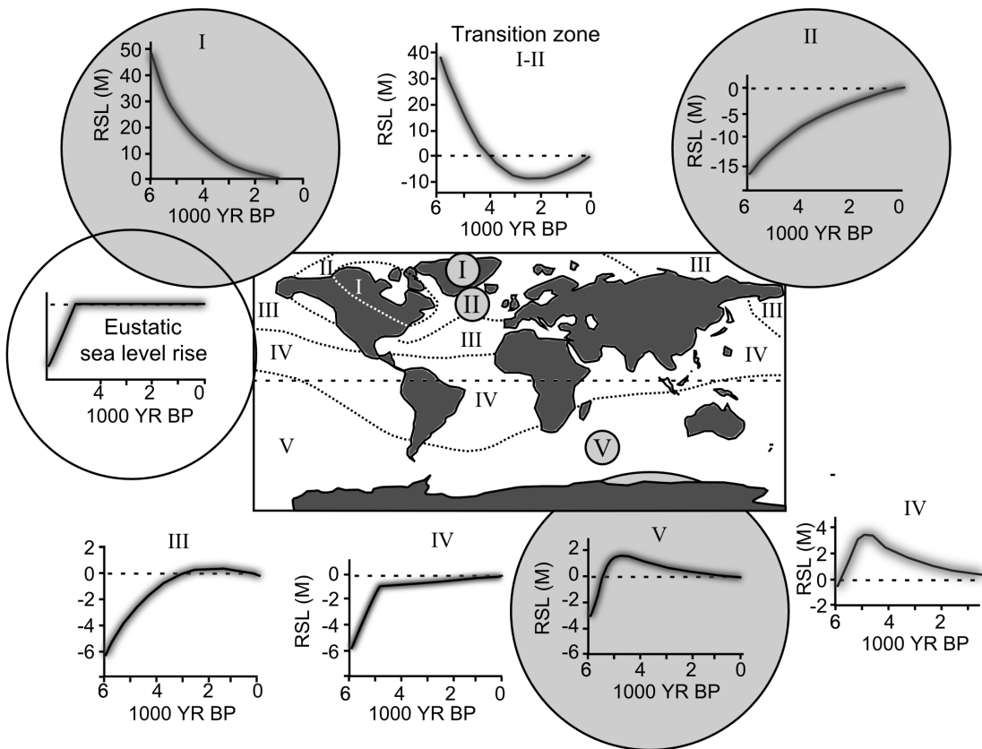
Figure 1: Local relative sea-level curves for the last 6000 years, modelled to include hydro-isostatic and glacio-isostatic effects combined with an idealised eustatic curve (after Clark and Lingle, 1979). Note the widely varying patterns of sea-level change at different places around the world, caused by deep-seated plastic flow in response to changing surface loads of ice and water.
