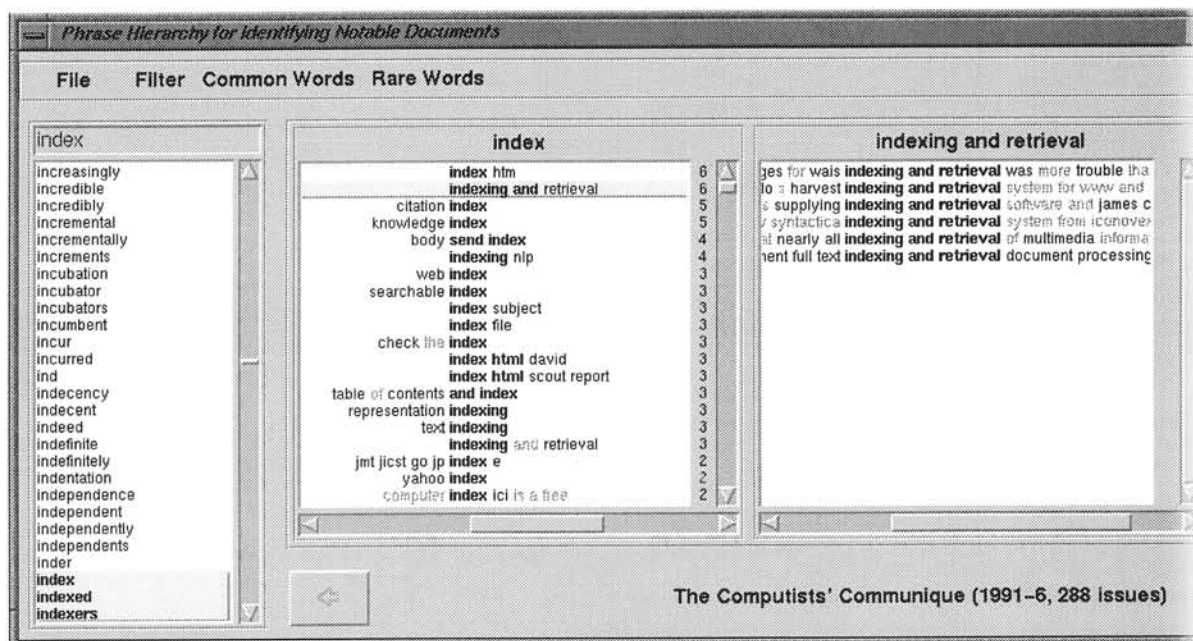
Figure 4 Part of a typical PHIND screen for the Computists' Communique collection
