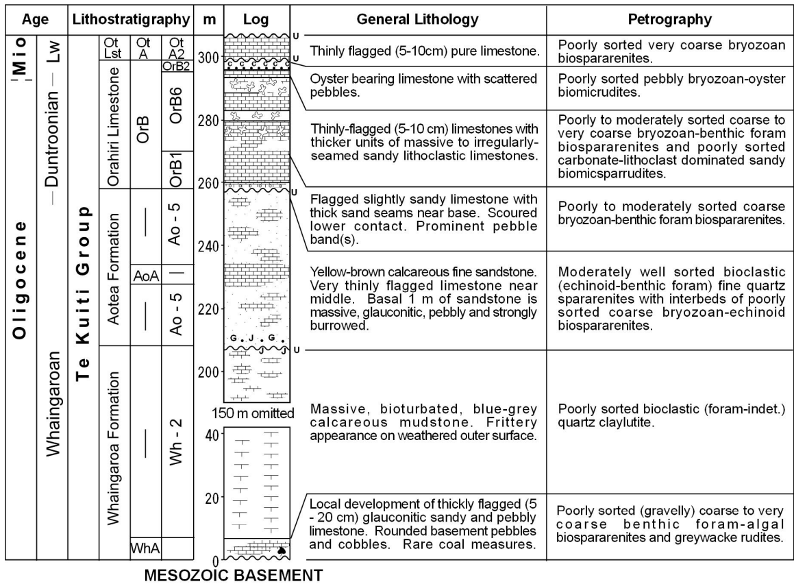
Fig. 20. Stratigraphic column for the Te Kuiti Group at Awakino Tunnel. (From Fig. 4 in Nelson et al. 1994).
