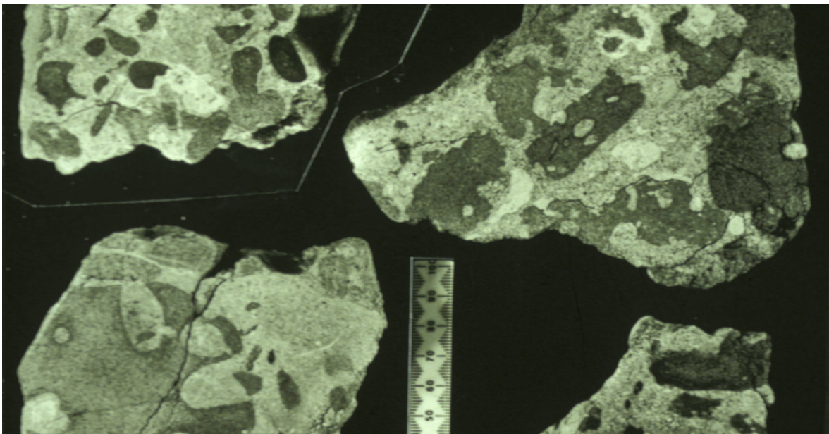
Fig. 23. Cut slabs of samples from redeposited (Limestone-in limestone) beds within Orahiri Limestone at Awakino Tunnel, showing pholad-bored and occasional red algal encrusted lithoclasts. (From Fig. 6 in Nelson et al. 1994).
