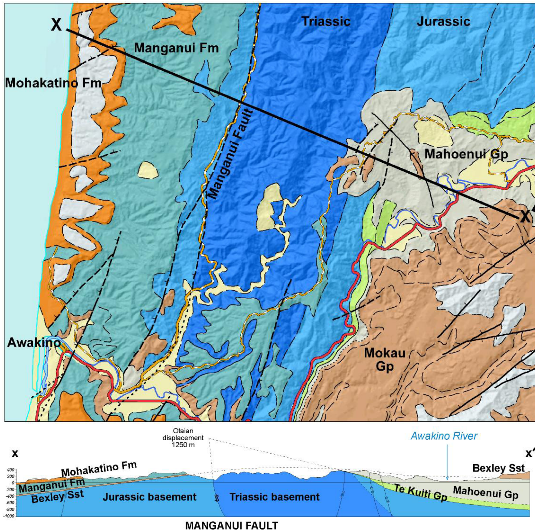
Fig. 19. Geological map and cross-section of the southern end of the Herangi Range. Based on map in Edbrooke (2005).
