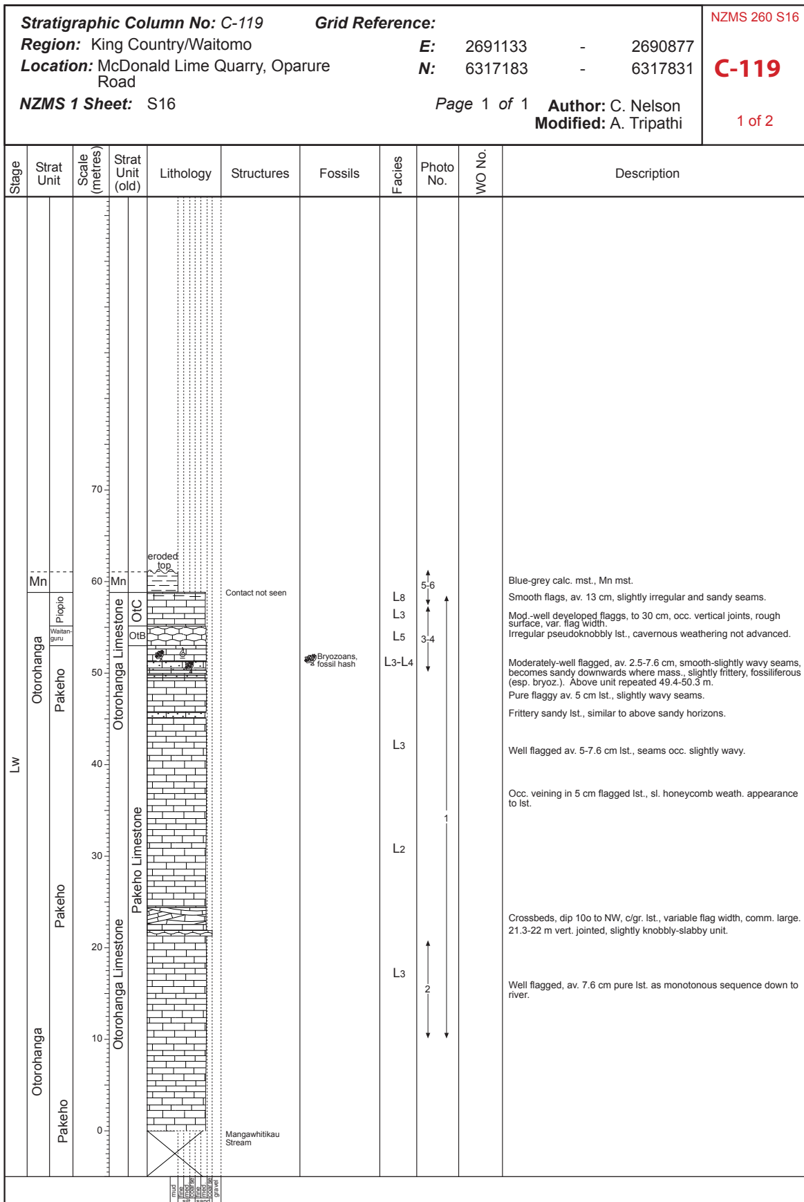
Fig. 12A. Stratigraphic column C119, McDonald Lime Quarry, Oparure. Facies codes are defined in Kamp et al. (2008). Photo numbers refer to those shown in Fig. 12B. (From Kamp et al. 2008).
