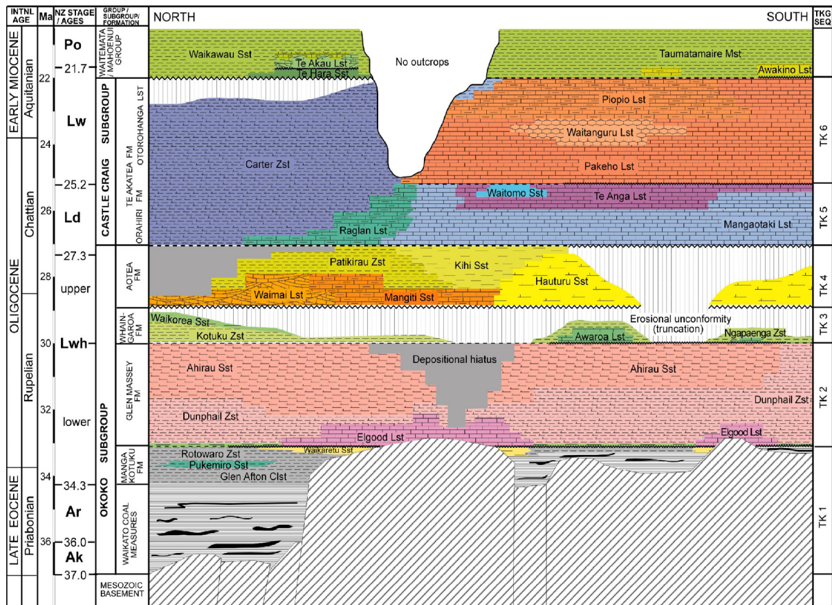
Fig. 11. N-S lithostratigraphic nomenclature for formations and several members in the Te Kuiti Group between the Waikato (in N) and King Country (in S) Basins, plotted within a chronostratigraphic panel. Note also the transition up into Waitemata (in N) and Mahoenui (in S) Group formations of Otaian (Po) age. (From Tripathi et al. 2008).
