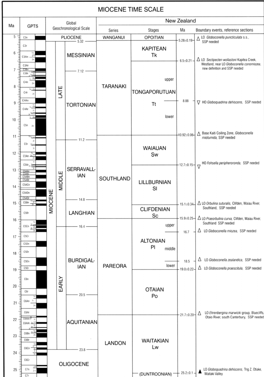
Fig. 4. Miocene time scale showing the age of New Zealand Stages. (From Fig. 12.1 of Crundwell et al. in Cooper (ed.) 2004).
