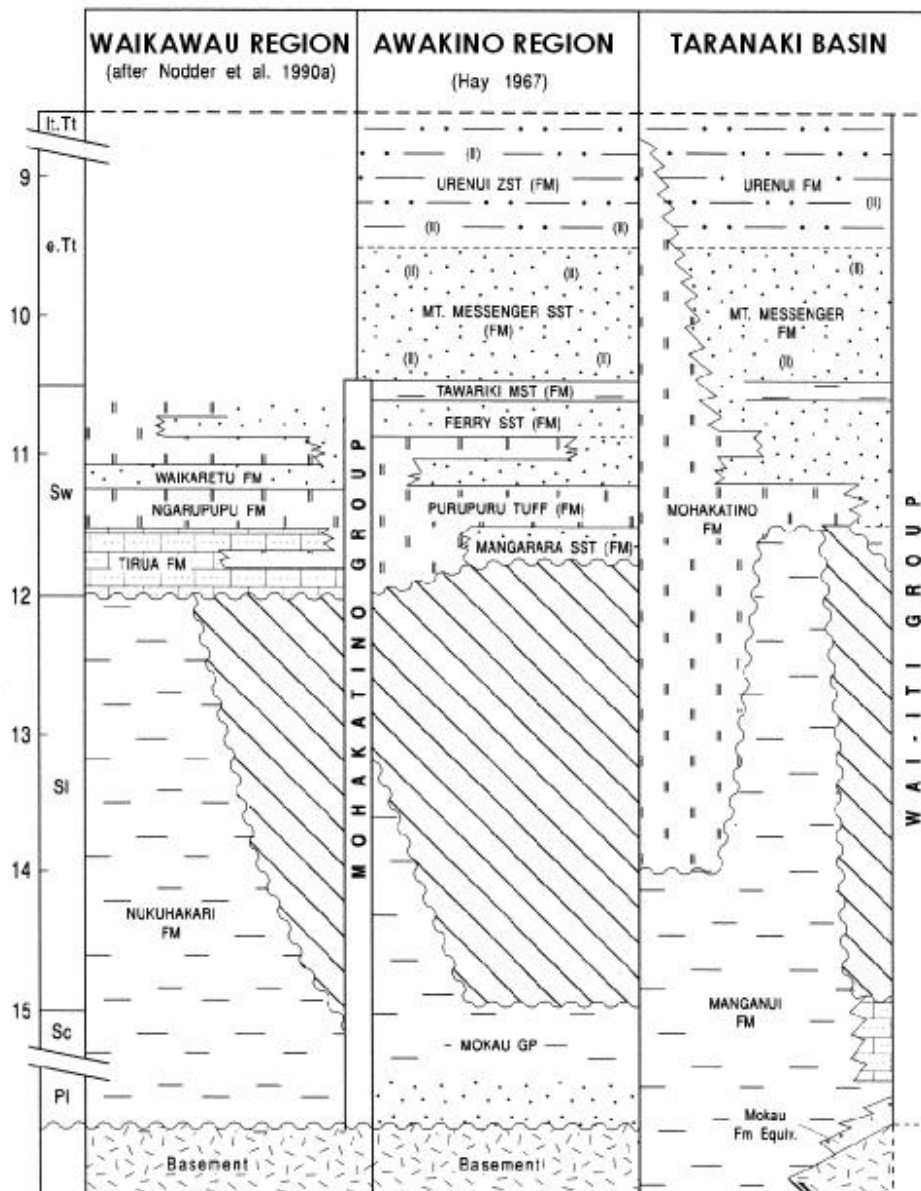
Fig. 27. Miocene time-stratigraphic logs for the Awakino region in relation to the Waikawau area to the north along the King Country coastline and offshore parts of Taranaki Basin. Mangarara Sandstone is shown for Awakino as being of Waiuan (Sw) age, but King et al. (1993) noted it contains Clifdenian (Sc) microfauna. (From King & Thrasher 1996).
