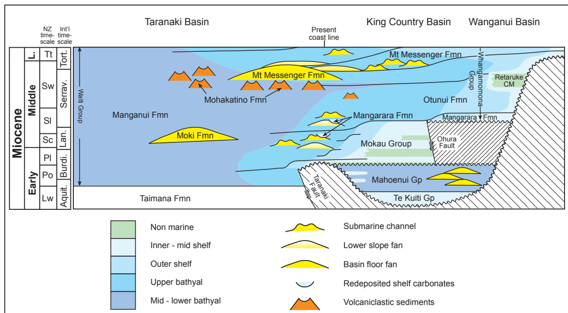
Fig. 10. Time-space stratigraphic panel for early and middle Miocene deposits and their inferred depositional settings in a roughly east (King Country Basin) to west (Taranaki Basin) section across the western North Island coastline. (From Fig. 2 in Puga-Bernabéu et al. 2009).
