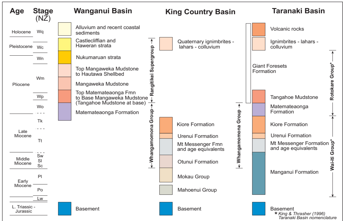
Fig. 5. The major Neogene stratigraphic units in each of Taranaki, King Country and Wanganui Basins, and their age. The Moki and Mohakatino Formations, which occur within Manganui Formation in Taranaki Basin, are not shown. (From Fig. 3 in Kamp et al. 2004).
