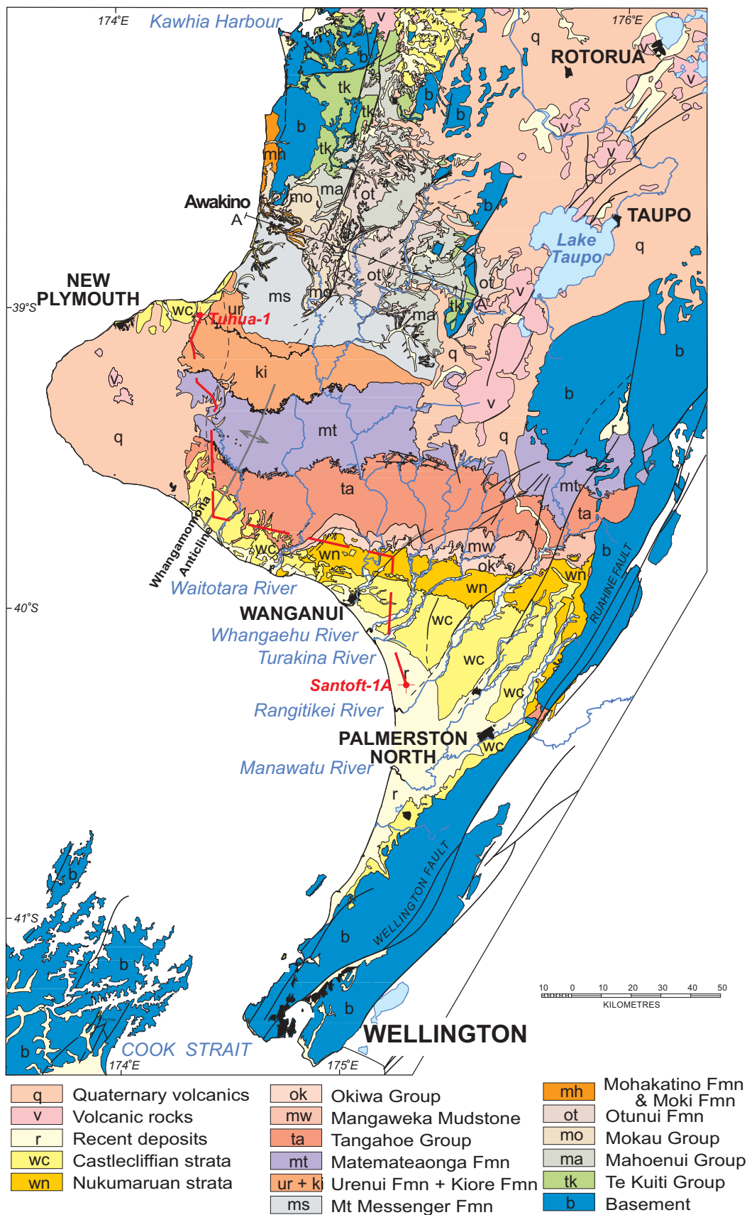
Fig. 2. Simplified geological map of western North Island (modified from New Zealand Geological Survey 1972), showing the main stratigraphic units in the eastern Taranaki, King Country and Wanganui Basins (located in Fig. 6). Cross-section line A-A' is the basis for the chronostratigraphic panel in Fig. 9. (From Fig. 1 in Kamp et al. 2004).
