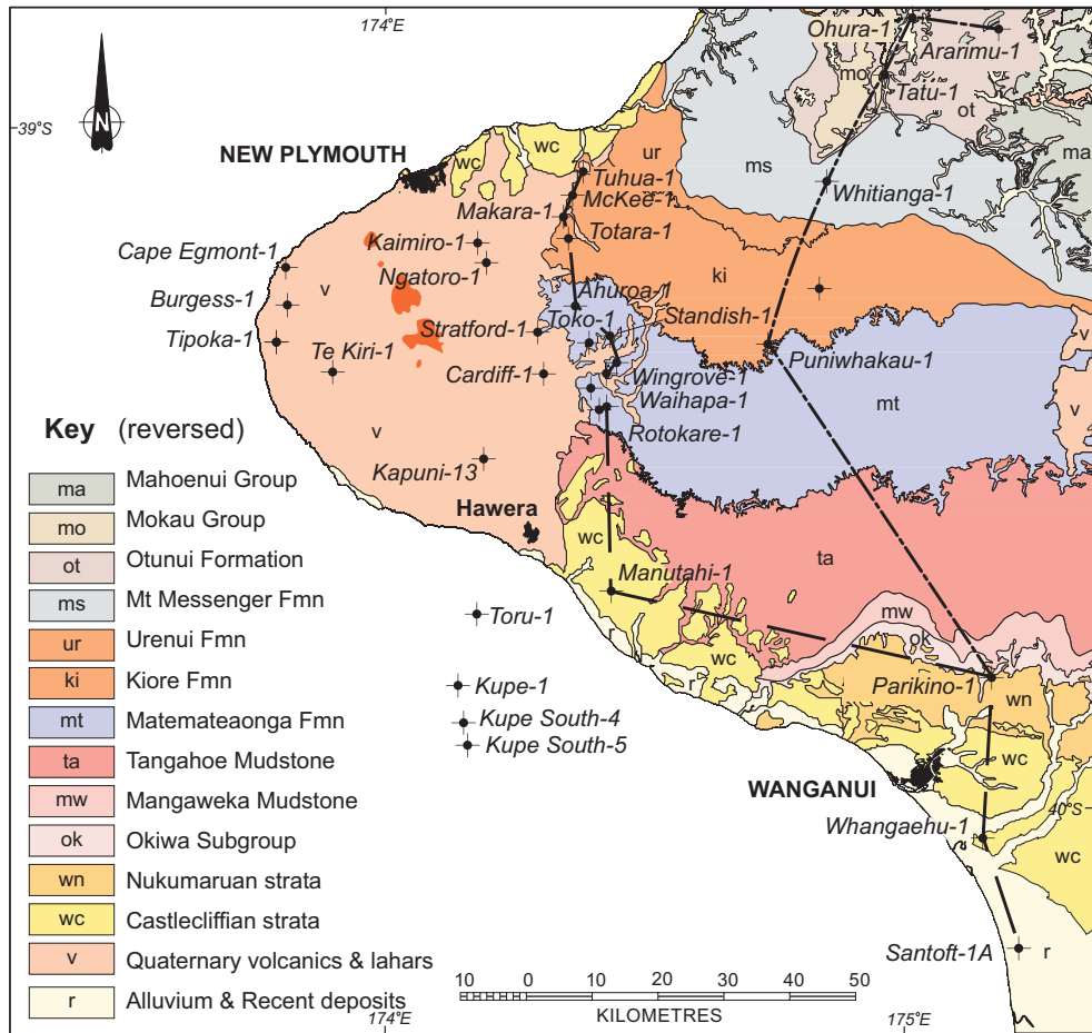
Fig. 7. Geological map of central-western North Island, including Taranaki Peninsula, showing the location of some key hydrocarbon exploration holes and the line of the N-S cross-section between King Country and Wanganui Basins illustrated in Fig. 8. (Modified from Fig. 5 in Kamp et al. 2004).
