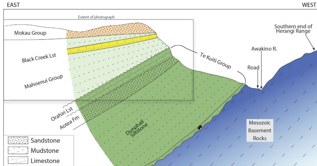
Fig. 17. Sketch illustrating the stratigraphy and structure of the Te Kuiti, Mahoenui and Mokau Groups in relation to basement at the northern end of Awakino Gorge. The inset box shows the approximate extent of the photo composite illustrated in Fig. 16. (From Fig. 12 in Kamp et al. 2004).
