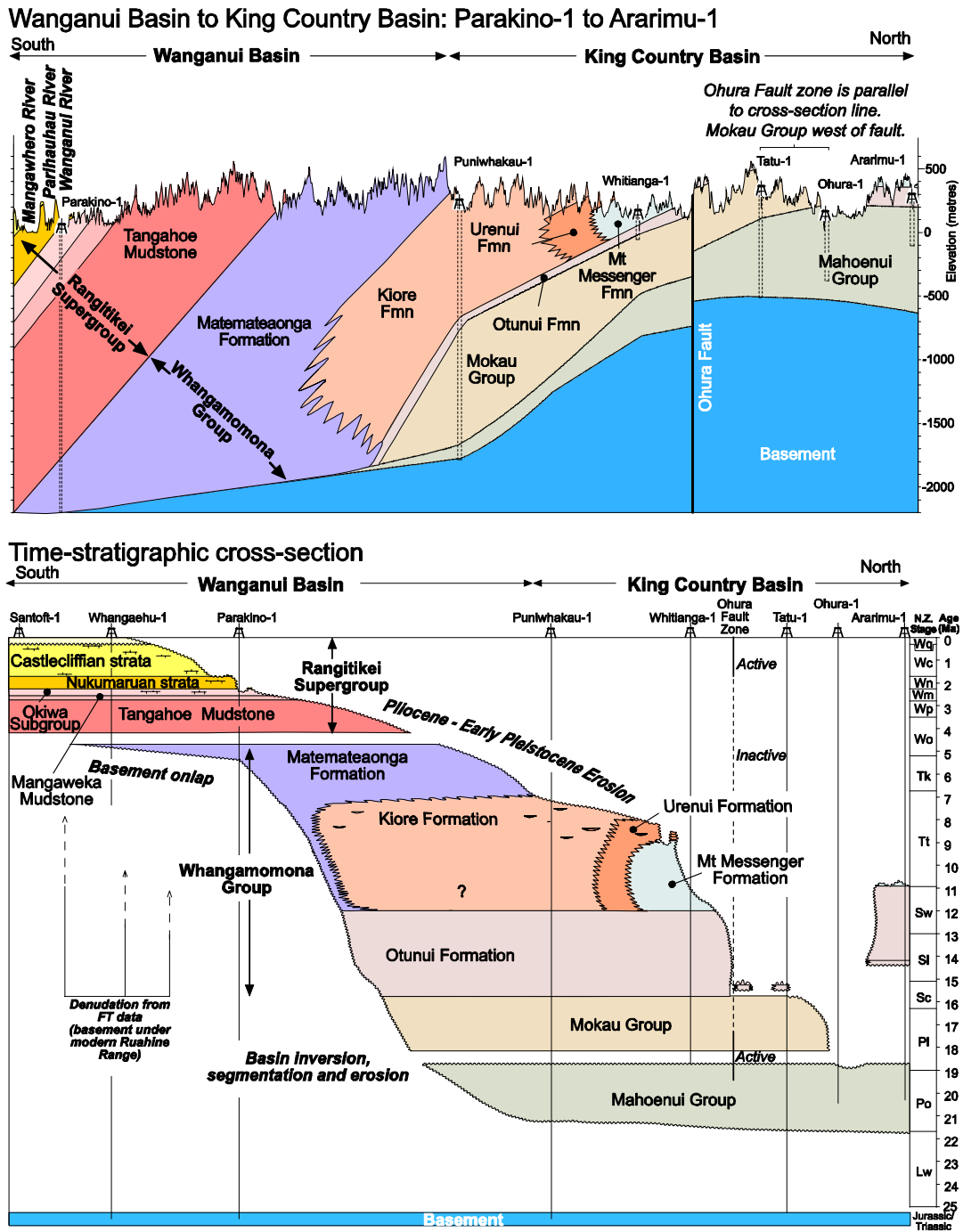
Fig. 8. Wanganui Basin to King Country Basin (Parakino-1 to Ararimu-1) stratigraphic panel (upper) built up from well-to-well correlations, and related time-stratigraphic cross-section (lower). The timing of denudation of basement underlying the present Ruahine Range, determined from apatite fission track analysis, is also shown. (From Fig. 6 in Kamp et al. 2004).
