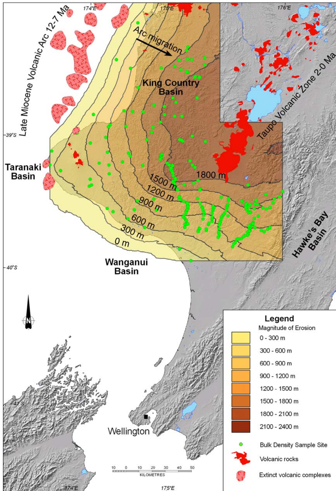
Fig. 6. Map showing the magnitude in 300 m contours and pattern of Pliocene-Pleistocene erosion over central North Island derived from mudstone bulk density data. See text for discussion. (From Fig. 4 in Kamp et al. 2004).
