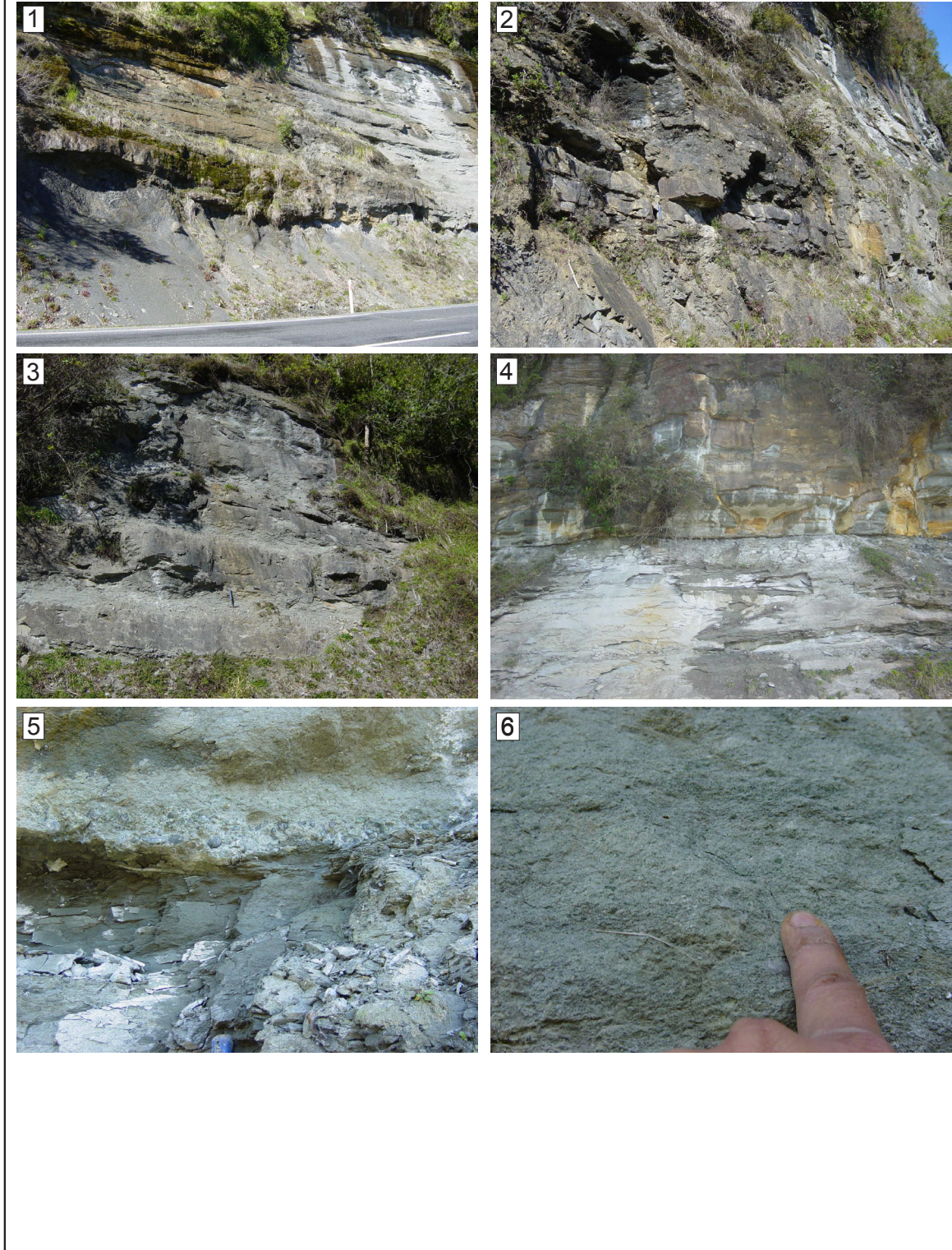
Fig. 15B. Field photos of locations at C166 identified on Fig. 15A.
