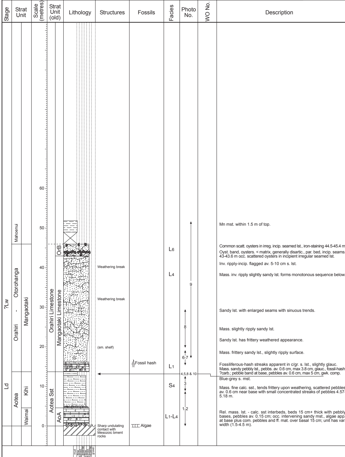
Fig. 15A. Stratigraphic column C166, Mangaotaki Bridge. Facies codes are defined in Kamp et al. (2008). Photo numbers refer to those shown in Fig. 15B (From Kamp et al. 2008).
