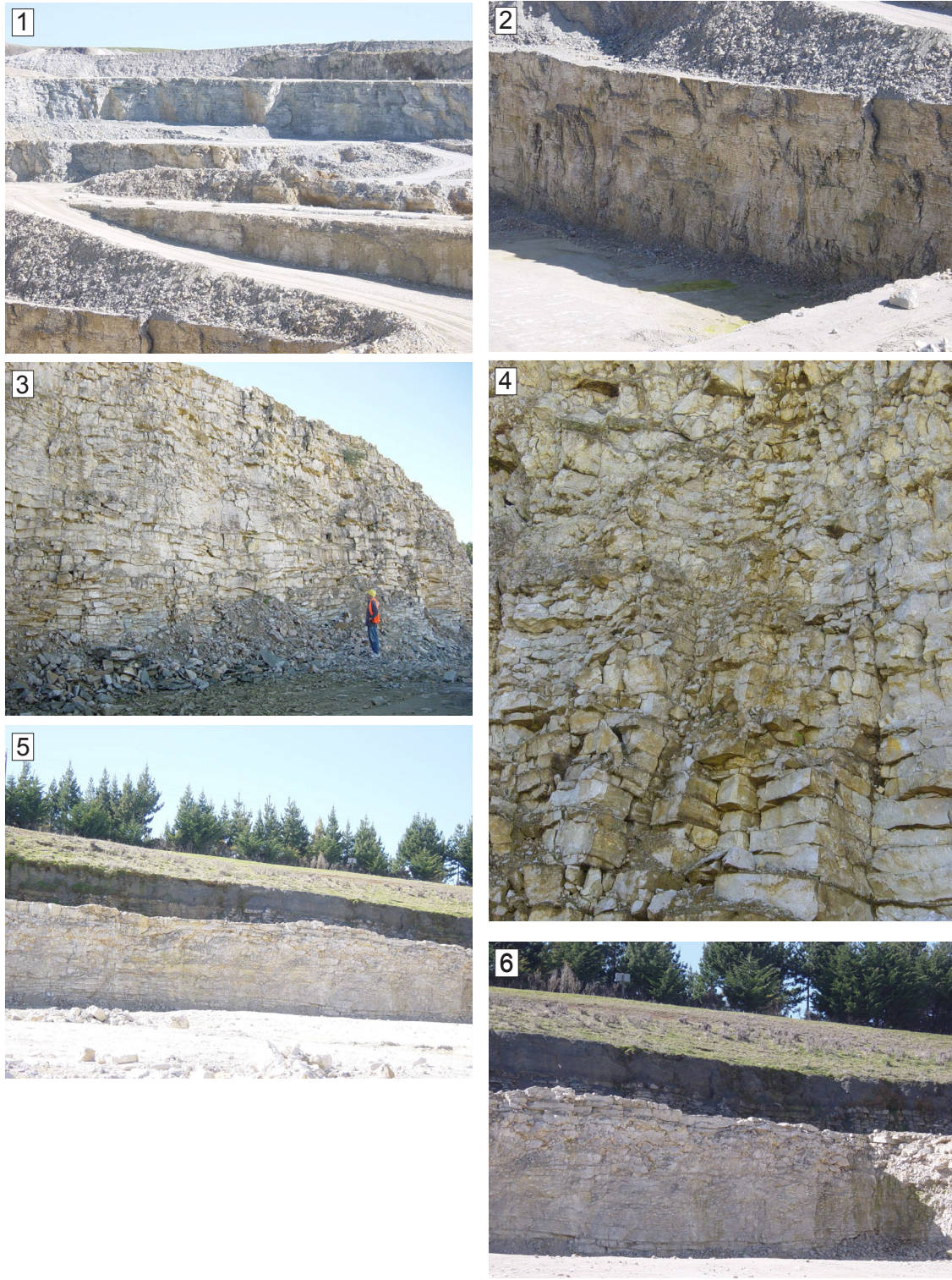
Fig. 12B. Field photos of locations at C119 identified on Fig. 12A.
