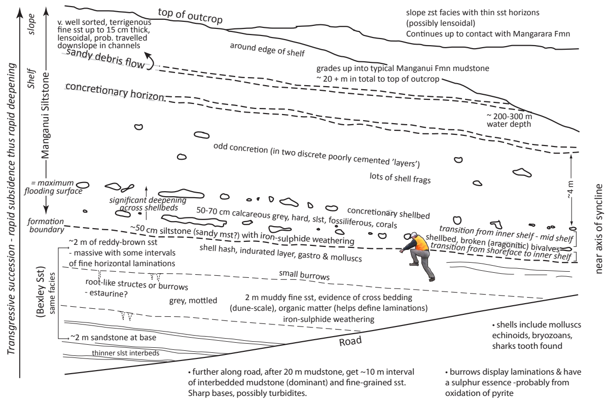
Fig. 26. Sketch stratigraphic section across the Bexley Sandstone to Manganui Formation transition near Awakino (compiled by Dr Rochelle Hansen, University of Waikato).
