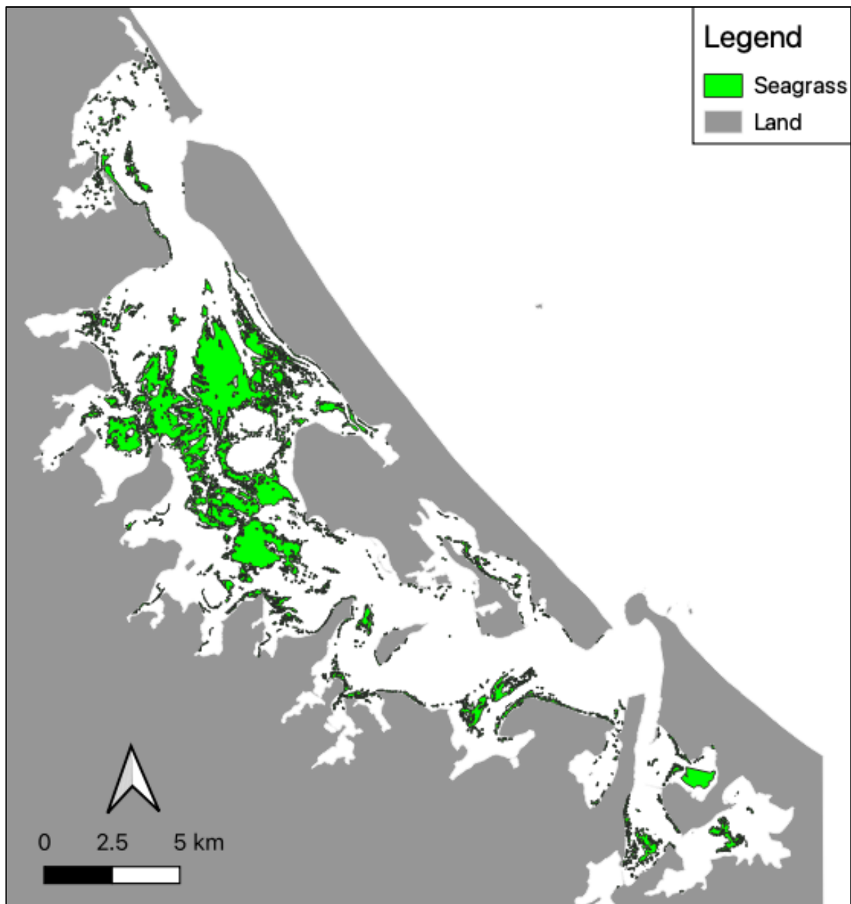
Figure 9 Seagrass extent in Tauranga Harbour in winter 2022.
