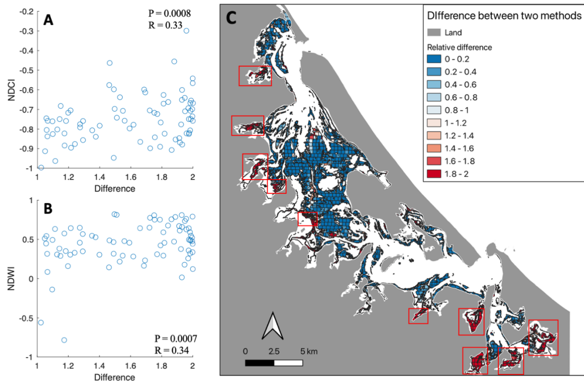
Figure 8 The correlation between NDCI, NDWI and difference of seagrass extent in the sub-estuaries from two methods (a & b) as well as the spatial distribution of relative difference map in the whole harbour.
