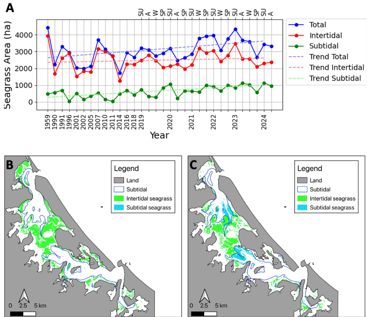
Figure 6 The extent of seagrass in the intertidal and subtidal regions from 1959 to 2024 with trendlines (a) and distribution maps of seagrass in the intertidal and subtidal regions in 2011 (b) and 2024 (c). The extent of seagrass was calculated seasonally from 2019.
