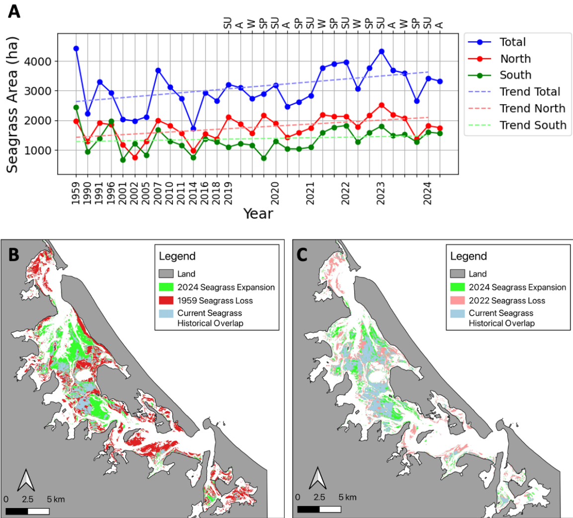
Figure 5 The extent of seagrass from 1959 to 2024 with trendlines (a) and change in seagrass extent between 1959 and 2024 (b) and between 2022 and 2024 (c). The extent of seagrass was calculated seasonally from 2019 (Summer: SU; Autumn: A; Winter: W & Spring: SP). The trendlines were generated based on the seagrass extent during summer each year. Green = most recent expansion, Blue = current seagrass coverage that overlaps the reported historical coverage, Red/Pink = areas of seagrass loss between historical and current extent.
