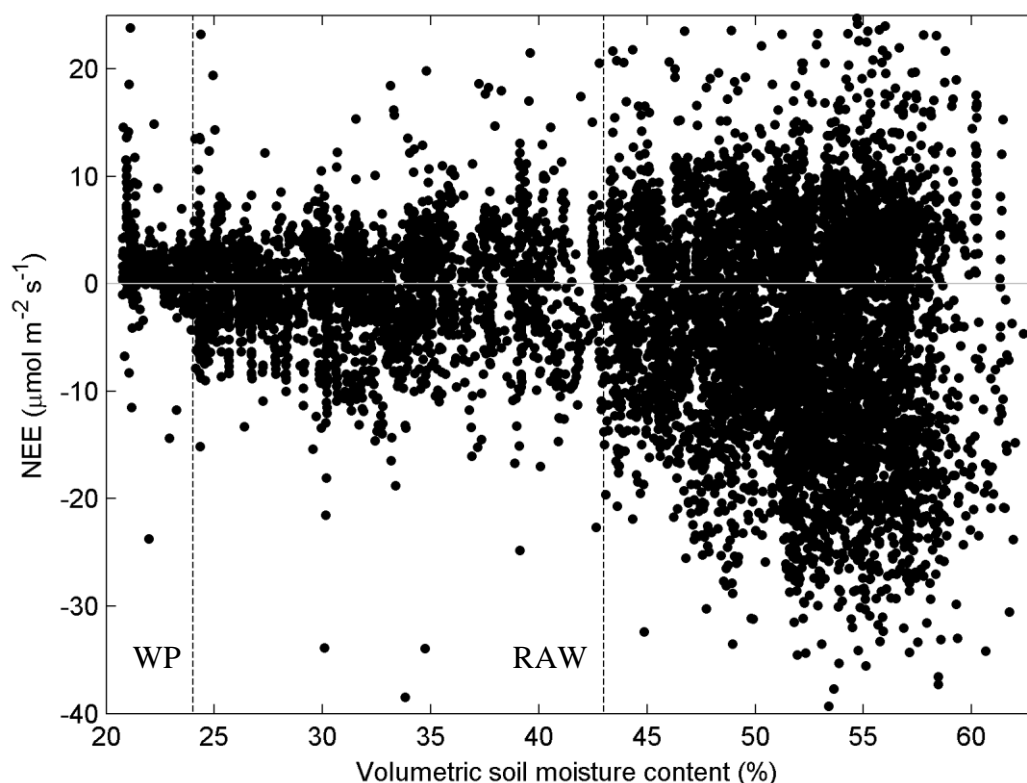
Fig. 4.3. Average 30 minute net ecosystem exchange of CO 2 (NEE) vs. volumetric soil moisture content for the entire dataset. The vertical dotted lines represent the lower limit of readily available water (RAW) and the wilting point (WP). RAW and WP thresholds derived from Singleton, (1991) for soils similar to the Matangi Silt loam.
