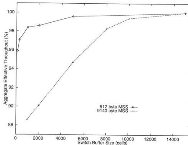
Figure 22 Effective Throughput vs. Switch Buffer Size
