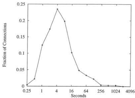
Figure 16 Distribution of TCP connection duration for WWW traffic
