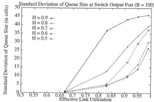
Figure 10 Standard deviation of queue size at switch output port for ethernet traffic (Chen, et. al., 1995)
