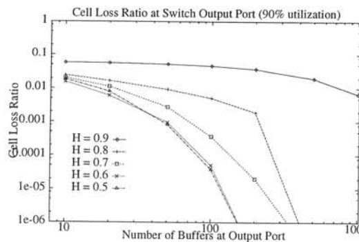
Figure 11 Cell loss ratio as a function of buffer size Traffic (Chen, et. al., 1995)
