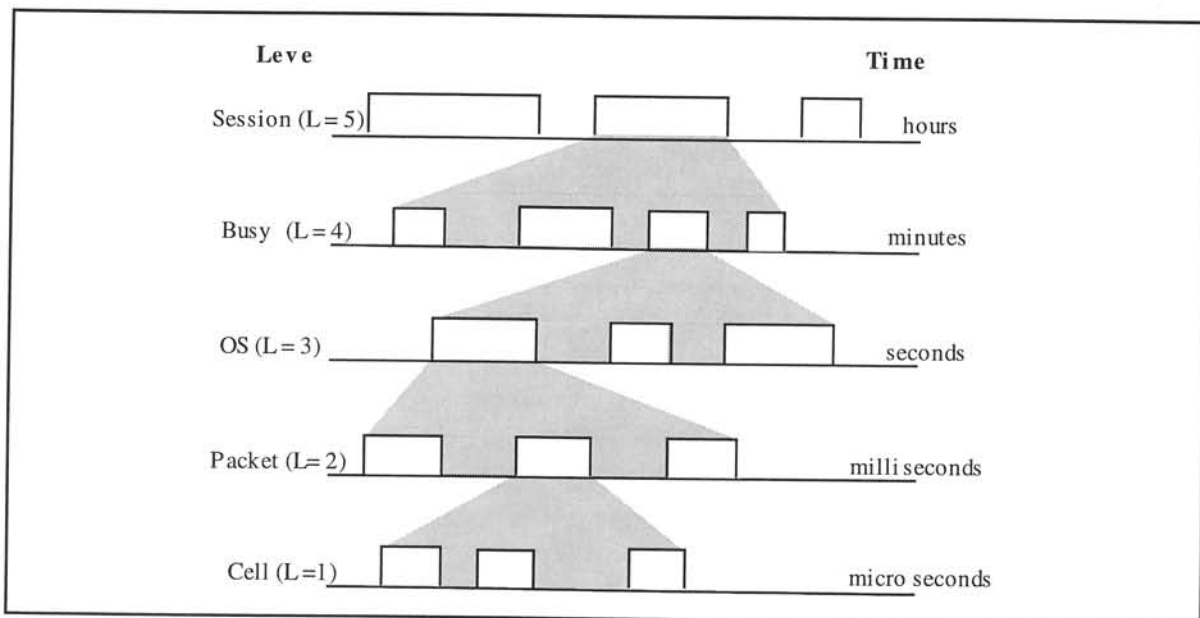
Figure 1 Multi-Layer States of Terminals
