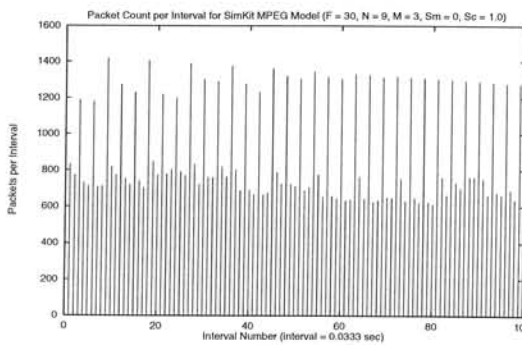
Figure 6 Packets per time interval for default MPEG GOP at 30 fps, no smoothing
