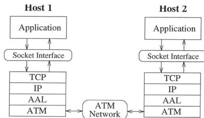
Figure 19 TCP over ATM protocol stack (Gurski and Williamson, 1995)
