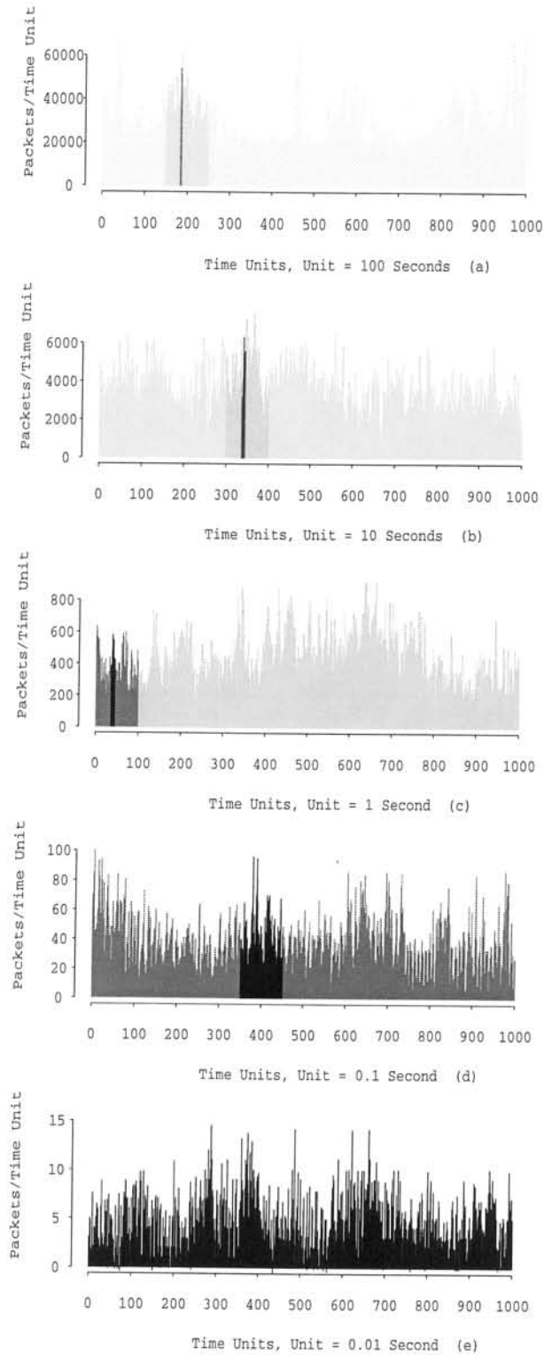
Figure 8 Pictorial “proof” of self-similarity: Ethernet traffic on 5 different time scales. (Different gray levels used to identify the same segments of traffic on the different time scales (Leland et. al., 1994))
