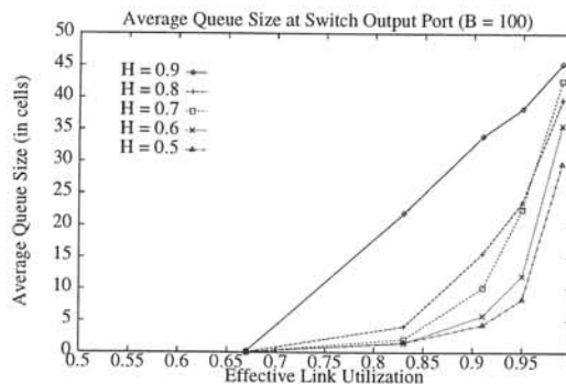
Figure 9 Average Queue Size at Switch Output Port for Ethernet Traffic (Chen, et. al., 1995)
