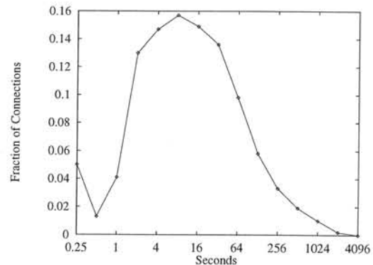
Figure 17 Distribution of TCP connection interarrival time for WWW traffic
