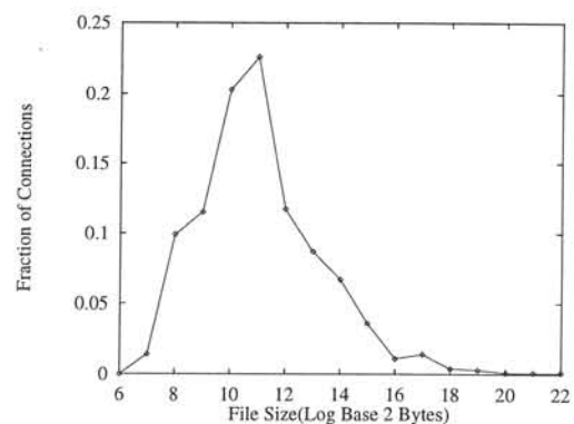
Figure 15 Distribution of bytes per TCP connection for WWW responses
