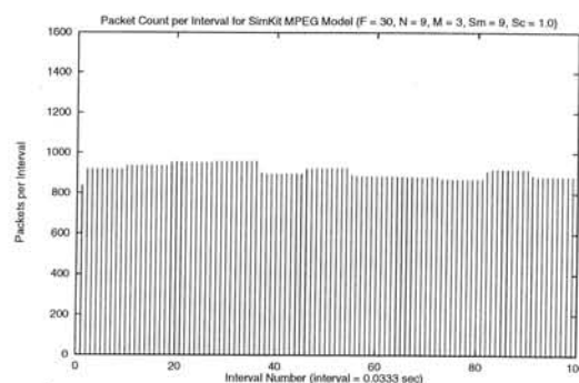
Figure 7 Packets per time interval for default MPEG GOP at 30 fps, smoothing = 9
