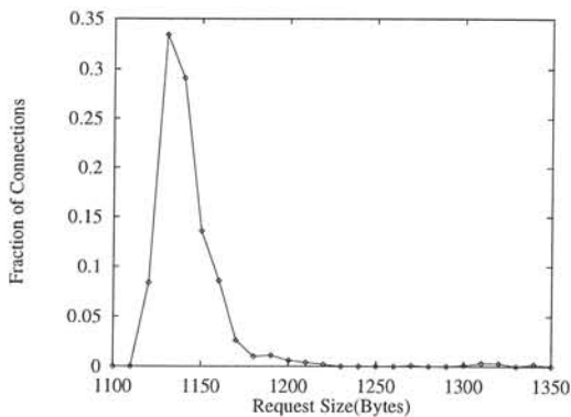
Figure 14 Distribution of bytes per TCP connection for WWW requests
