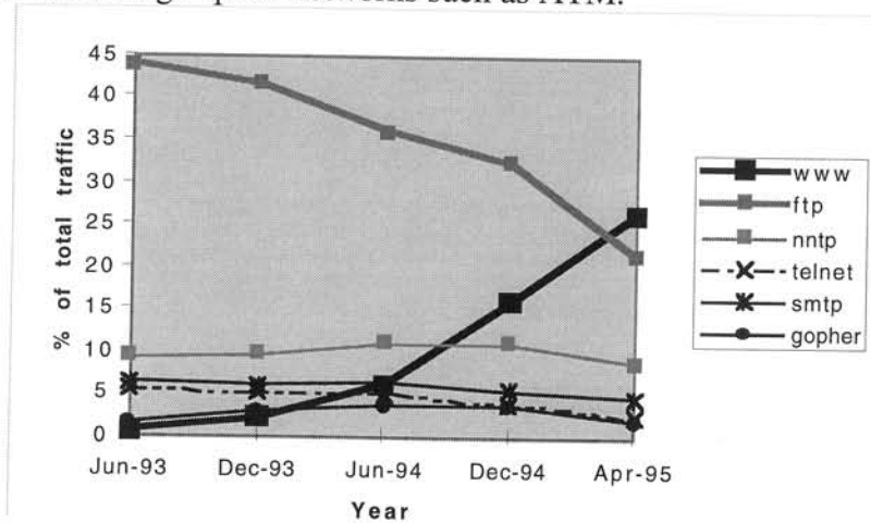
Figure 12 Percentage of total traffic on the Internet for the 6 largest contributors over time
