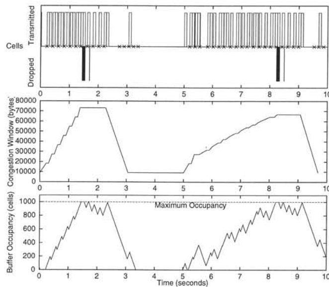
Figure 21 Dynamics of a Single TCP Source
