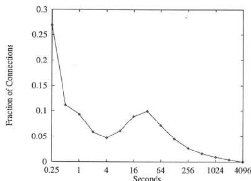
Figure 18 Distribution of TCP connection gap time for WWW traffic
