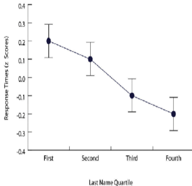
Figure X. Mean response time by the alphabetical position of respondents' names in the alphabet. Response times are expressed as z scores. Error bars represent standard errors.
