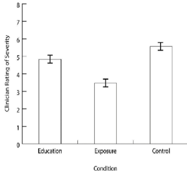
Figure X. Mean clinician's rating of phobia severity for participants receiving the education treatment and the exposure treatment. Error bars represent standard errors.
