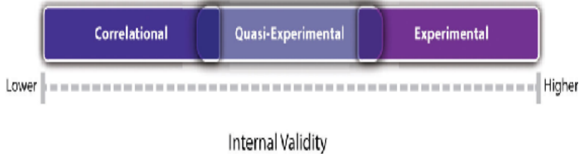
Figure 7.1 Internal Validity of Correlation, Quasi-Experimental, and Experimental Studies. Experiments are generally high in internal validity, quasi-experiments lower, and correlation studies lower still.
