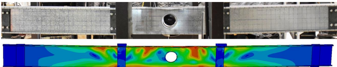
(f) W240-L4-UH5
