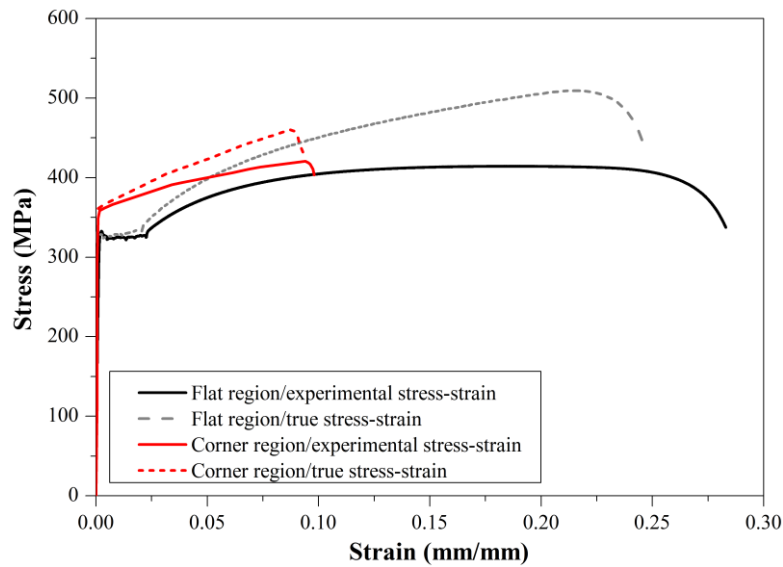
Fig. 5 Stress-strain curves of flat and corner coupons (Section 240) [13]
