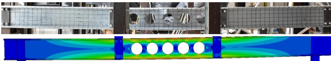
(f) W240-L4-UH5
