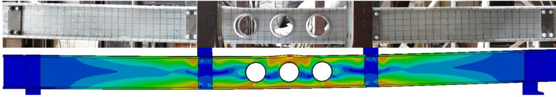
(b) W240-L4-EH3
