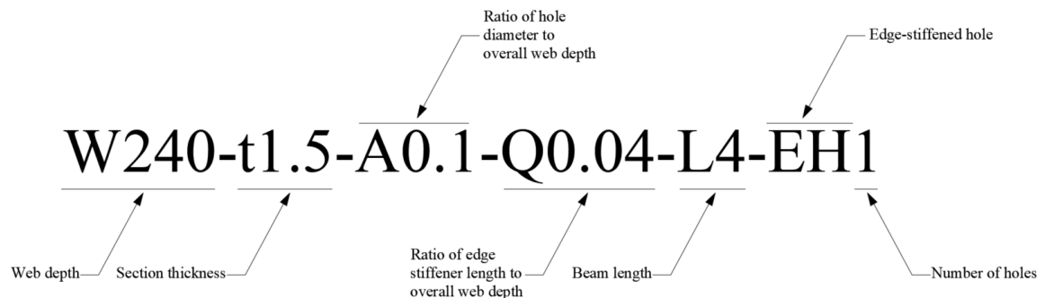
Fig. 12 Specimen labelling
