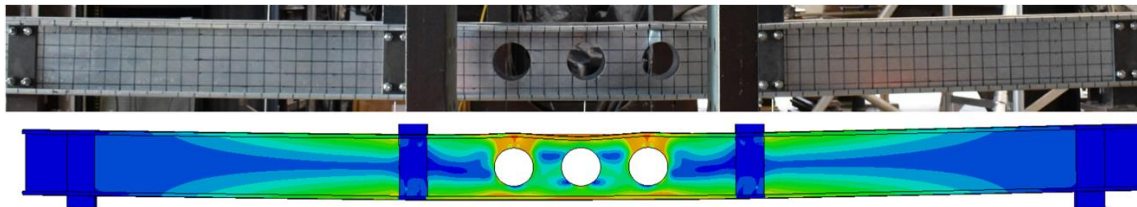
(e) W240-L4-UH3
