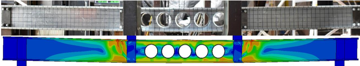
(c) W240-L4-EH5
