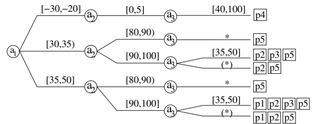
Figure 1. Profile tree for Example 1
