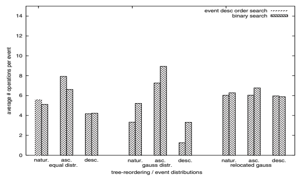
(b) Experiment TA2: small differences in attribute distributions
