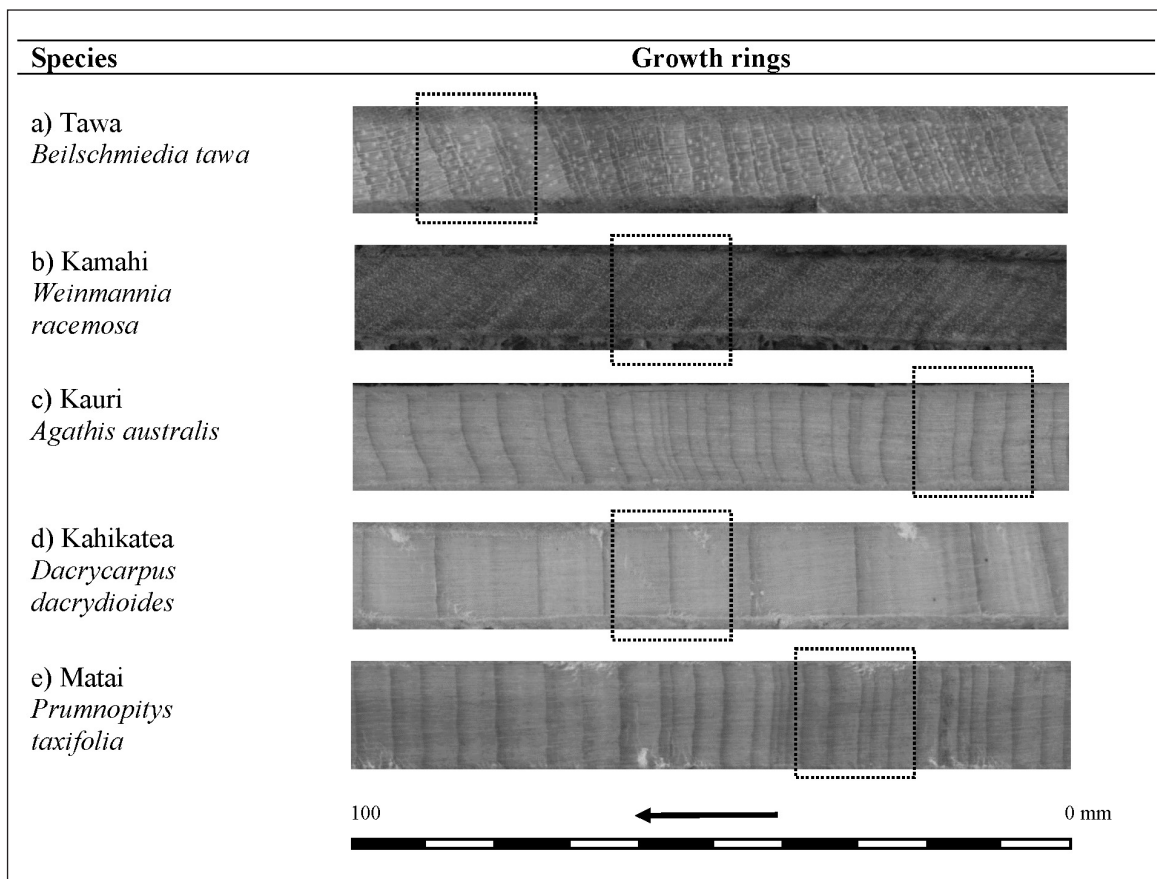
Figure 2. Growth rings of selected species. Particular characteristic features are highlighted (boxes): Tawa ( Beilschmiedia tawa ) can have ambiguous parenchyma bands forming apparent ring boundaries; Ring boundaries of kamahi ( Weinmannia racemosa ) are indistinct; Density fluctuations in kahikatea ( Dacrycarpus dacrydioides ), kauri ( Agathis australis ) and matai ( Prumnopitys taxifolia ) growth rings may be misinterpreted as true growth rings. The arrow indicates direction of growth from inner to outer rings.
