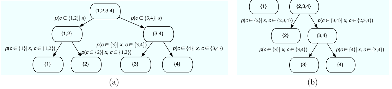
Figure 1. Two different systems of nested dichotomies for a classification problem with four classes.
