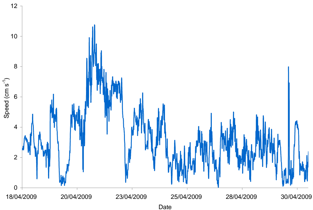
Figure 9. Velocity of water currents near the lake bed at LAKE 2 from 17 April to 1 May, 2009. Wind came mainly from the north-easterly quarter on 19 April and 24-30 April 2009 and south to south-easterly directions (Figures 10 and 12). The fastest wind speeds recorded
