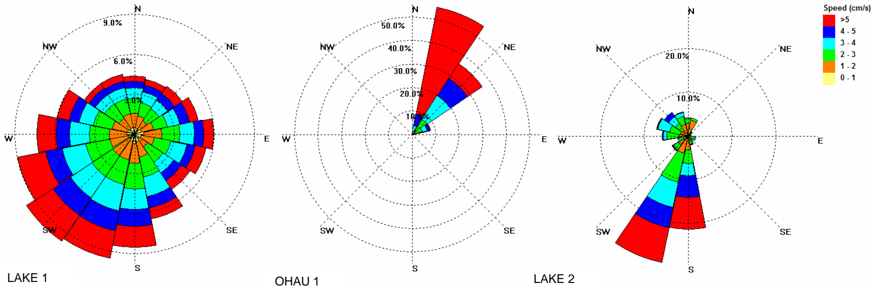
Figure 5. Water current speeds and directions through the water column at LAKE 1 and immediately above the lake bed at sites OHAU 1 and LAKE 2, 17 April to 1 May 2009. Inset is a schematic map of the Okere Arm.
