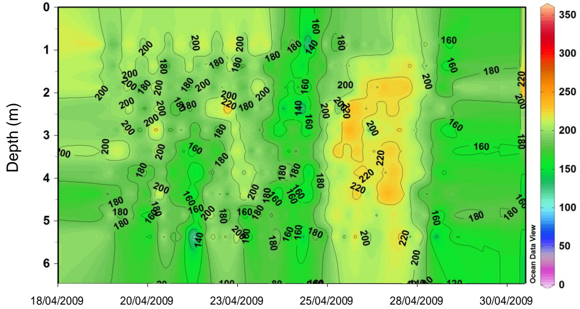
Figure 6. Direction of water currents through the water column at LAKE 1 from 17 April to 1 May, 2009.
