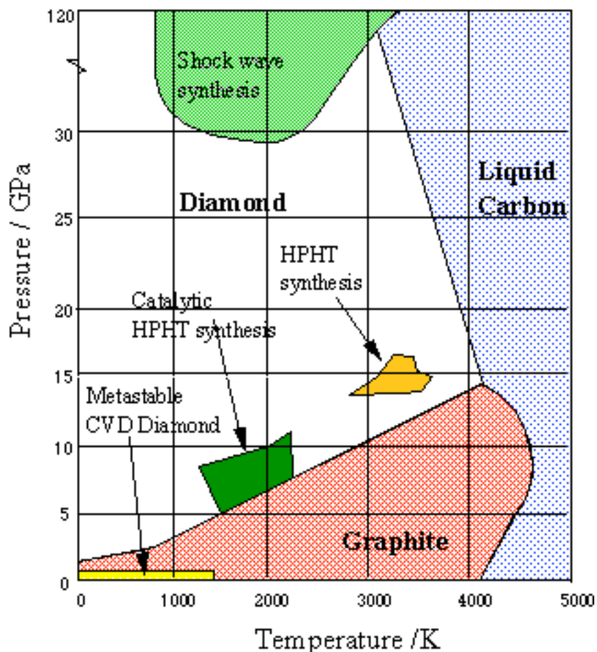
Figure 15. The phase diagram for diamond and graphite, depicting the pressure-temperature regions that correspond to the liquid and the two solid states of the element carbon. Note that the solid form known as diamond sits above the solid form known as graphite on the pressure scale. Inset regions identify where various man-made processes lie. From Bundy (1980)
