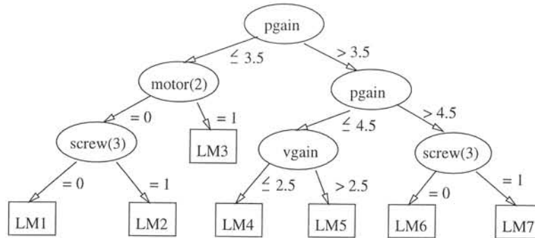
Fig. 2. Model tree for data set servo
